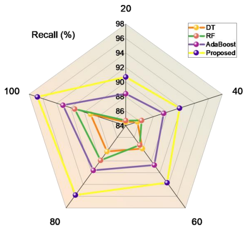
Figure 7. Recall
