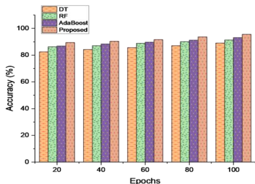
Figure 6. Accuracy
