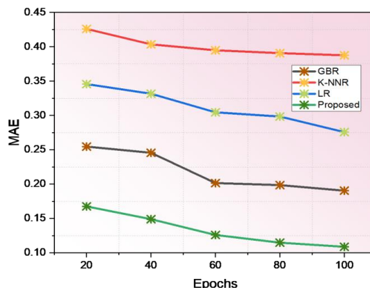
Figure 9. MAE
