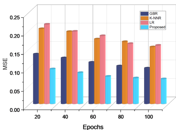
Figure 10. MSE
