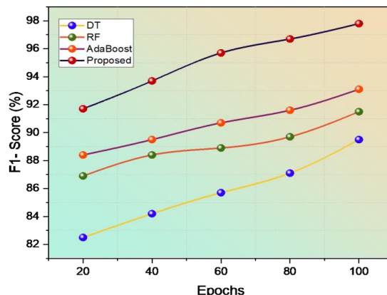
Figure 8. F1-score
