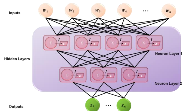
Figure 3. ANN structure
