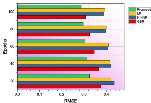
Figure 11. RMSE
