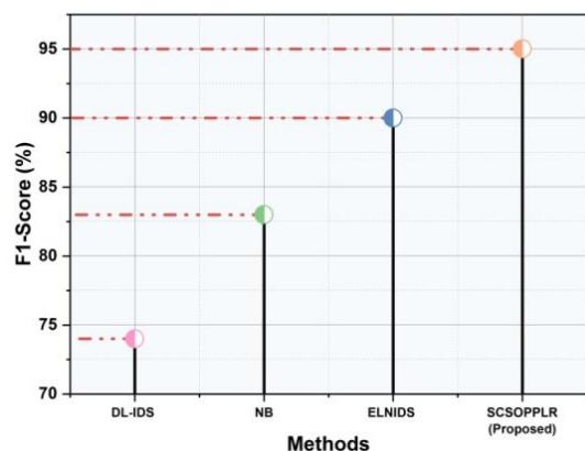
Figure 7. Comparison of F1-score
