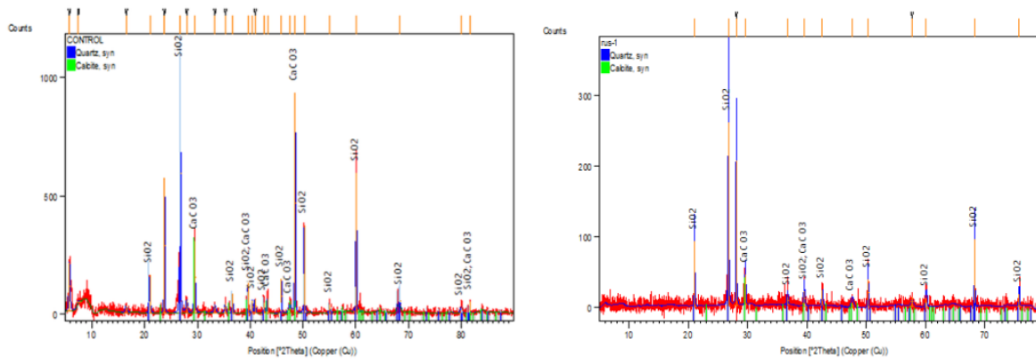
Figure 6. XRD graph of control and RUS-1 samples.
