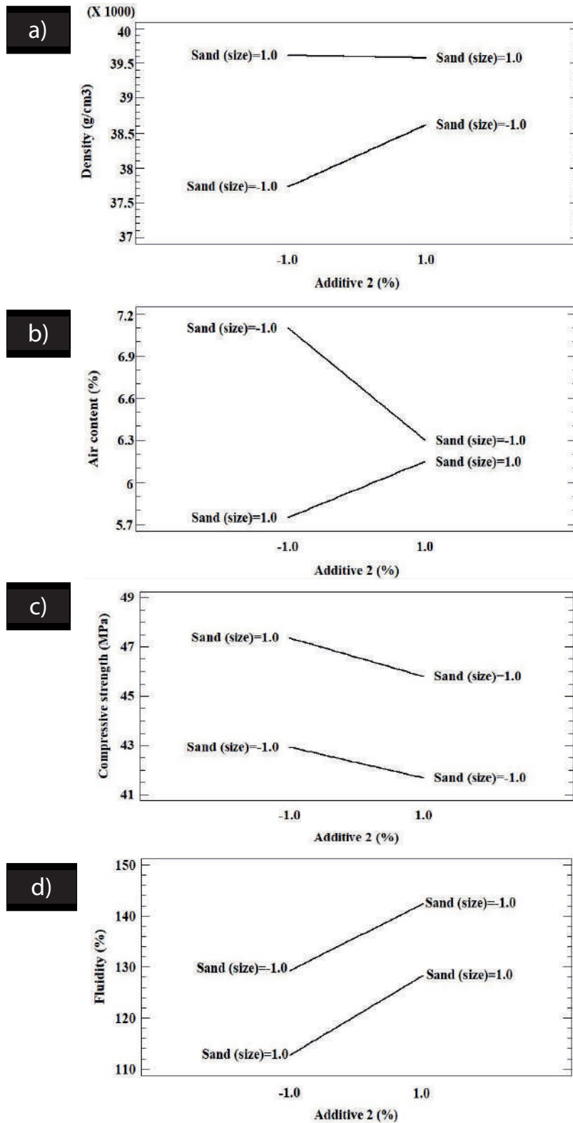
Figure 13. Interaction plots of factorial design B for a) density, b) air content, c) compressive strength, and d) fluidity
