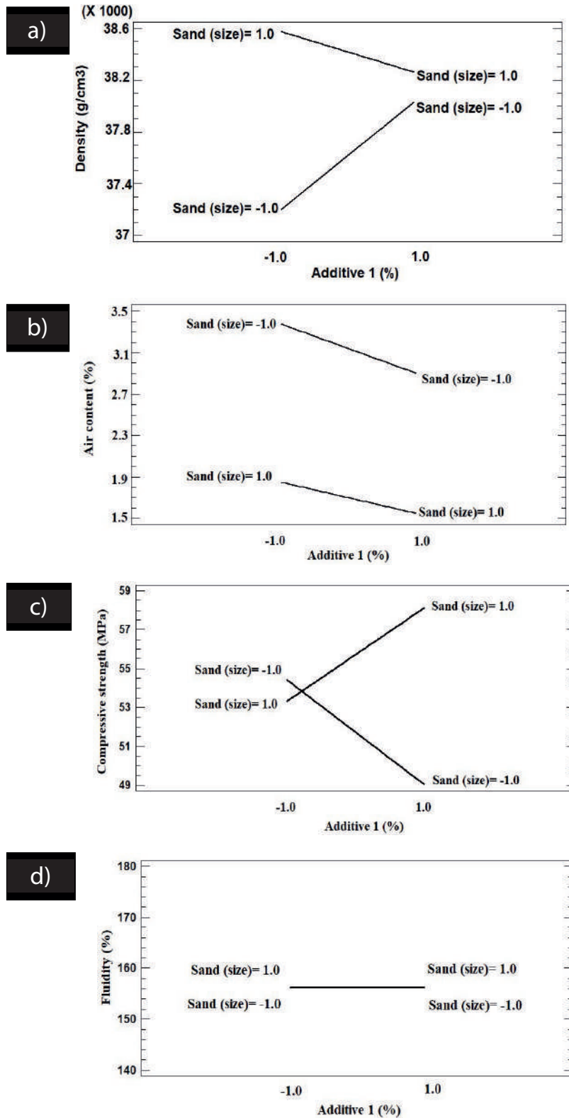
Figure 12. Interaction plots of factorial design A for a) density, b) air content, c) compressive strength, and d) fluidity
