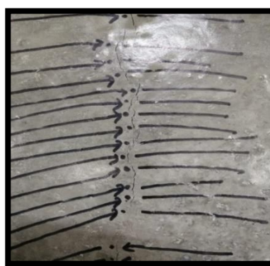
Fig. 11 Plastic shrinkage crack in concrete made with P-MF-0.20
