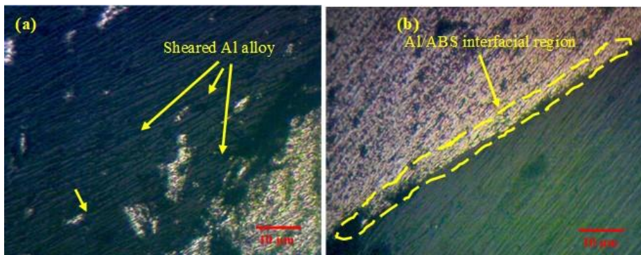
Fig. 5 Bonding Mechanisms in Hybrid Al/ABS Joints (a) Interlocked/Shear-Induced Bonding, (b) Adhesion Bonding
