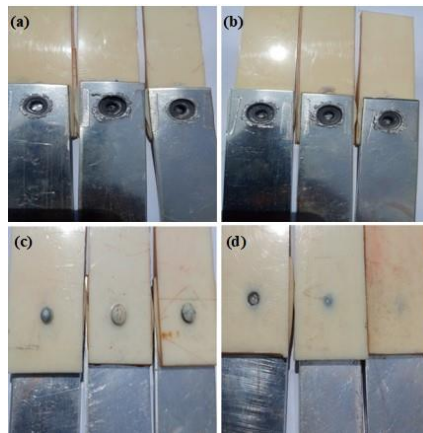
Fig. 4 Surface Appearances of Hybrid Al/ABS Joints, (a) Front Views of FSSW Joint, (b) Front Views of FSC Joint, (c) Back Views of FSC Joint, (d) Back Views of FSSW Joint
