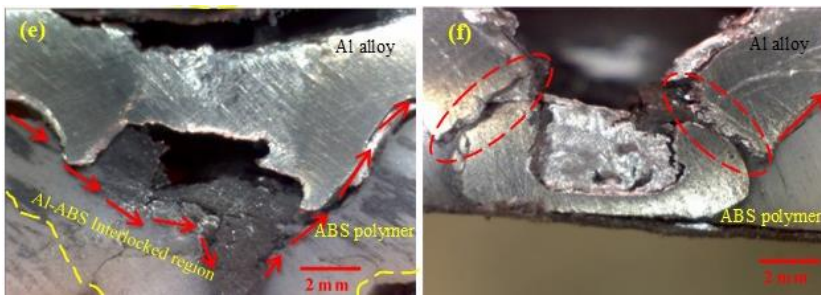
Fig. 10 Fracture Path of the FSC and FSSW Joints (a) Unbuttoning Fracture Mode in FSC, (b) Unbuttoning Fracture Mode in FSSW, (c) Circumferential-Partial Al in-Polymer Shearing Mode in FSC, (d) Circumferential-Partial Al in-Polymer Shearing Mode in FSSW Joint, (e) Mid-Nugget Shearing Mode in FSC, (f) Mid-Nugget Shearing Mode in FSSW Joint
