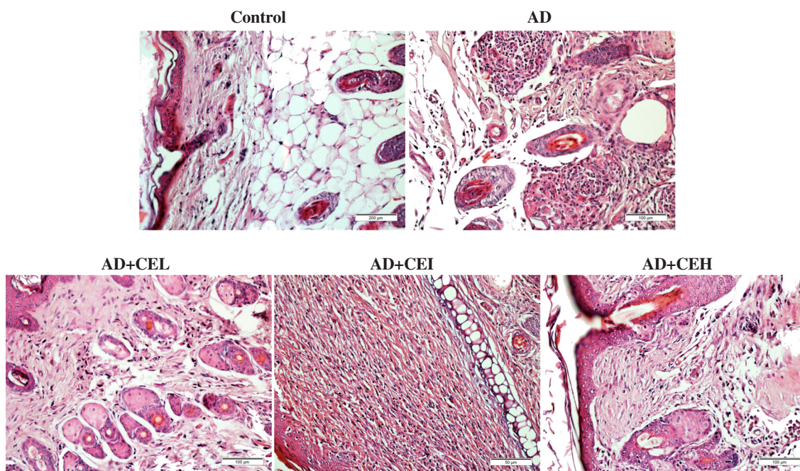
Figure 3. Effect of caraway on skin histology in AD mice. The skin from each mouse (collected on day 28) was fixed and embedded in paraffin. Sections (5-mm) were prepared and the tissues were then stained with H&E. The AD group shows severe inflammation and infiltration of immune cells into the skin compared to the control group. The caraway-treated groups dose-dependently reduce infiltration of inflammatory cells and signs of inflammation in the skin of mice. Magnification: ×20.
