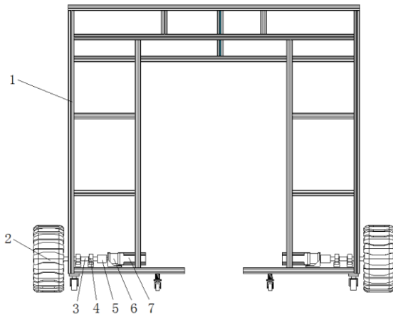
Fig. 2 - Schematic diagram of moving steering device
