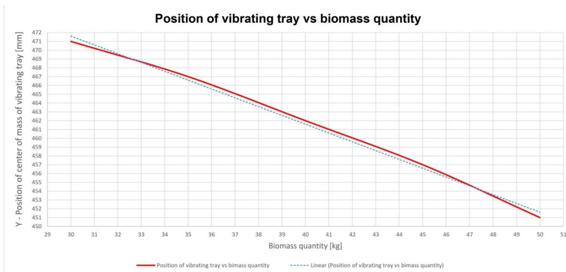
Fig.11 - Position of vibrating tray vs biomass quantity
