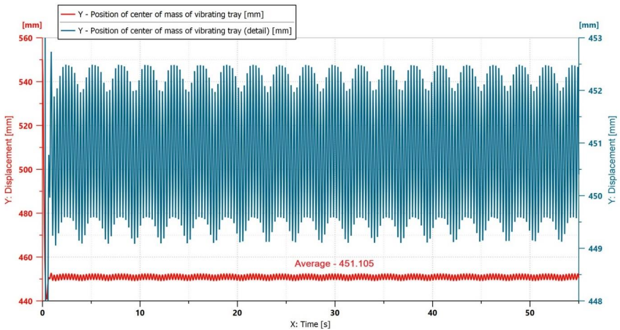
Fig. 5 - Y - Position of centre of vibrating tray mass (red) and in detail (blue)
