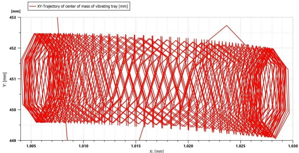
Fig. 6 - XY-Trajectory of centre of vibrating tray mass
