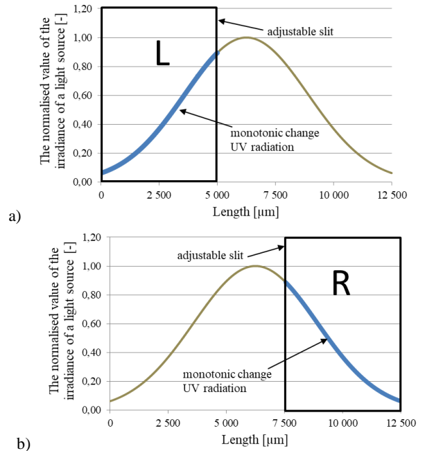
Fig. 3. Change of apodisation by means of a slot of adjustable width located on a) rising profile of the laser beam marked as L, b) falling profile of the laser beam R
