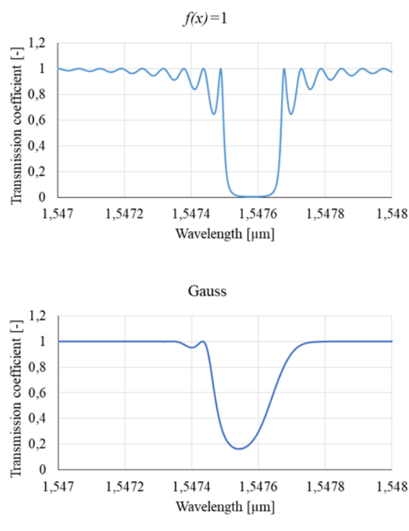
Fig. 1. Spectral characteristics of gratings with different apodisation functions: a) apodisation by f(x) = 1 , b) apodisation by Gaussian function
