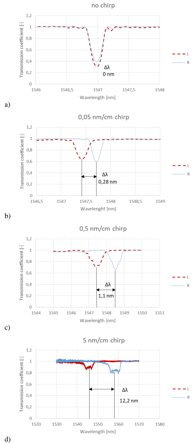
Fig. 7. Spectral characteristics of gratings produced in the laboratory, a) without chirp, b) with a 0.05 nm/cm chirp, c) with a 0.5 nm/cm chirp, d) with a 5 nm/cm chirp
