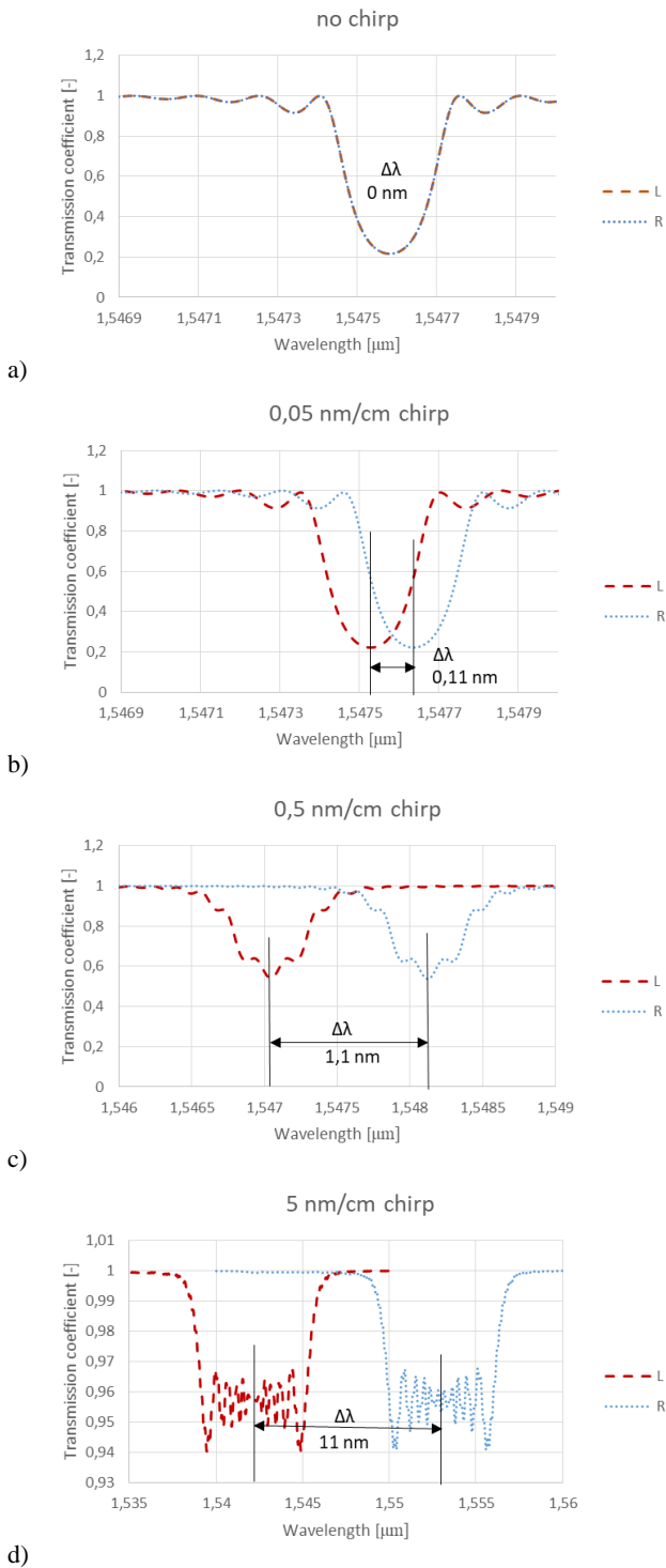
Fig. 6. Spectral characteristics of grids with apodisation profile f(x) = 1 , a) without chirp, b) with a 0.05 nm/cm chirp, c) with a 0.5 nm/cm chirp, d) with a 5 nm/cm chirp
