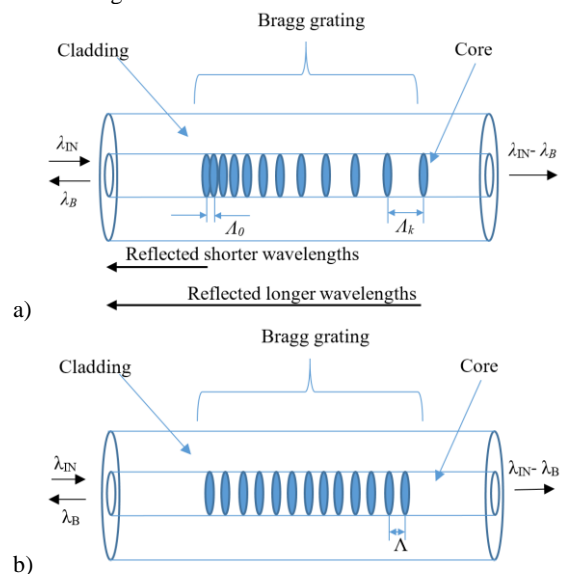
Fig. 4. Scheme and principle of operation of a fibre Bragg grating: a) with chirp, b) without chirp
