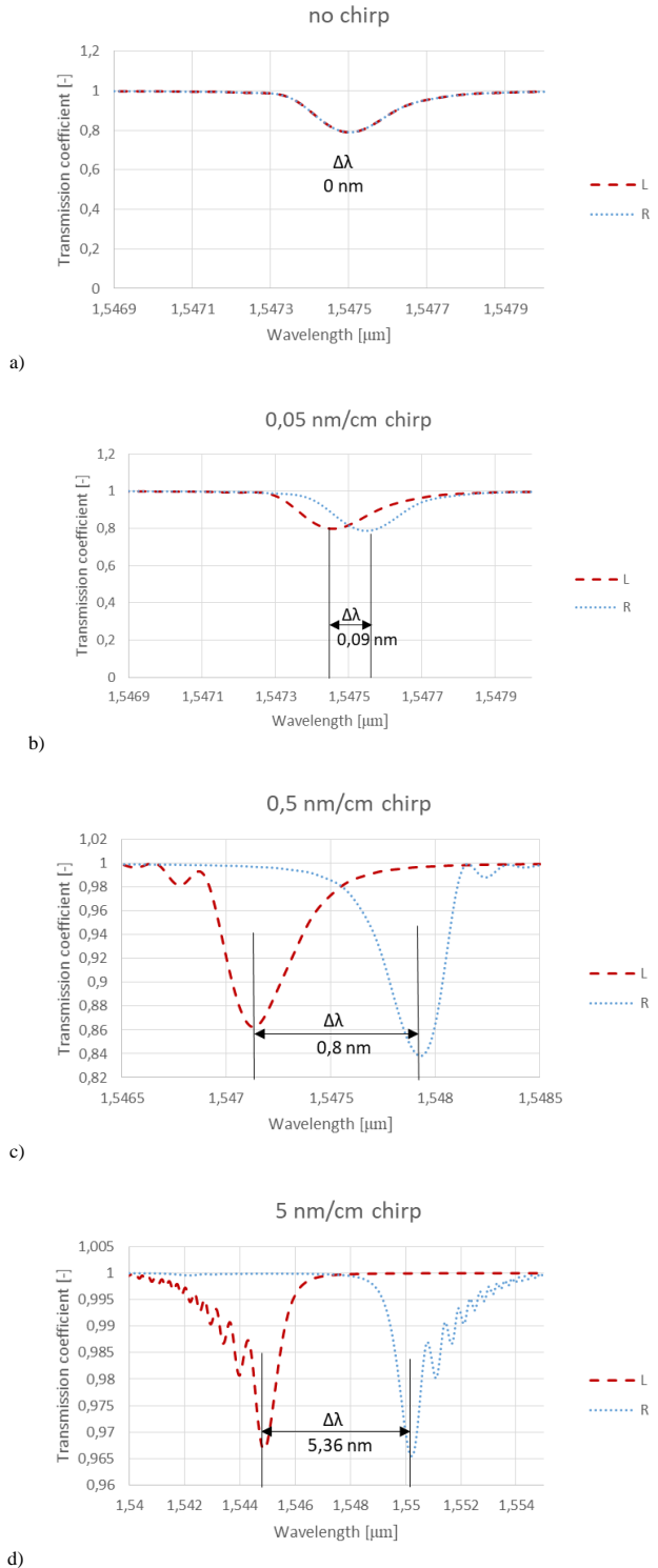
Fig. 5. Spectral characteristics of grids with Gauss apodisation profile, a) without chirp, b) with a 0.05 nm/cm chirp, c) with a 0.5 nm/cm chirp, d) with a 5 nm/cm chirp
