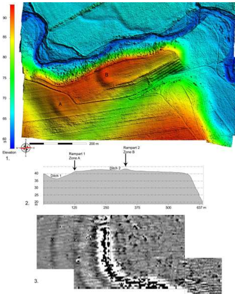
Fig. 23. Orbeasca de Sus-Cetate: 1. Digital model of the terrain (DSM type) 30 cm/pixel resolution created through photogrammetric algorithms applied to aerial images recorded with UAVs; 2. Elevation profile on DSM through its fortification elements; 3. Magnetic map (a square measures 30x30 m); black stands for highly magnetic and white for highly non-magnetic; X, Y, Z – magnetic, circular anomalies are very probably fortification ditches.
