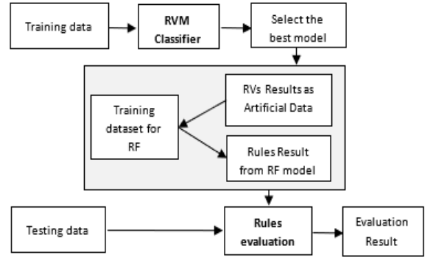
Figure. 4 The steps of proposed RVM_RF
