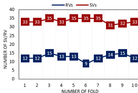
Figure. 6 Comparison of RVs and SVs number in each training fold
