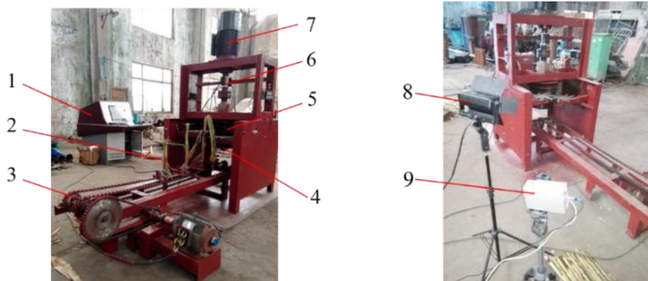
Fig. 7 - Stalk returning test rig
