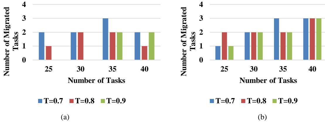
Figure. 5 Illustration of number of migrated loads of: (a) setup 1 and (b) setup 2
