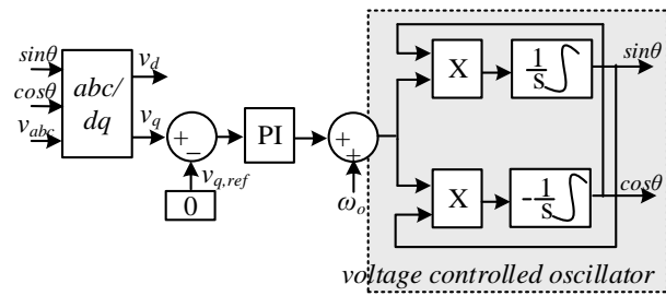
Figure. 6 SRF-PLL structure
