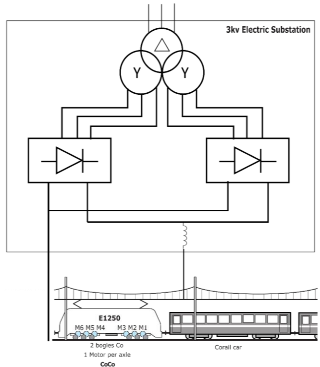
Figure. 1 The locomotive E1250 connected to Corail train
