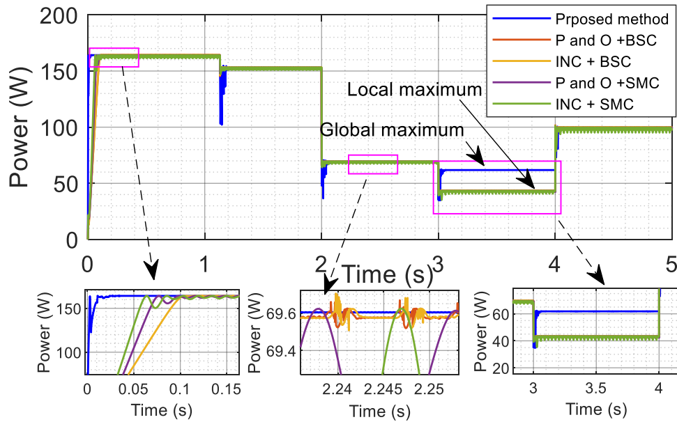
Figure. 6 PV power at the terminals o PV panel by using the P&O-SMC, P&O-BSC, INC-SMC, INC-BSC and PSO-SMC
