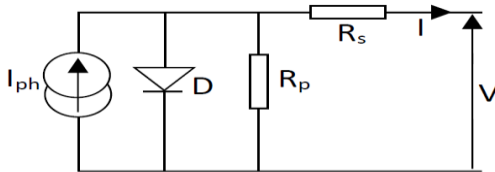
Figure. 2 PV cell
