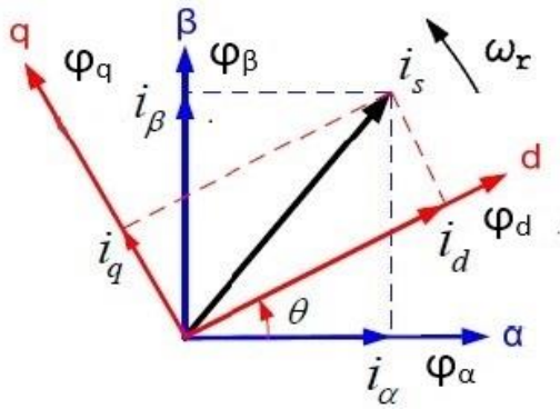
Figure.1 Orientation of different reference frame
