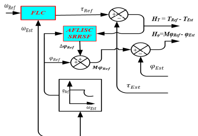
Figure.4 Block diagram of proposed control technique
