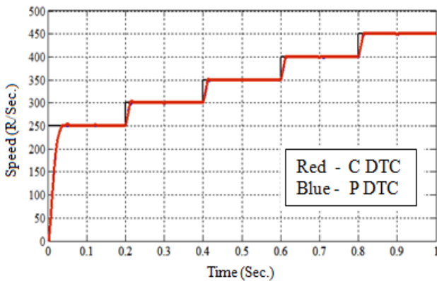
Figure. 7 Comparison of speed of CDTC and PDTC for IPMSM
