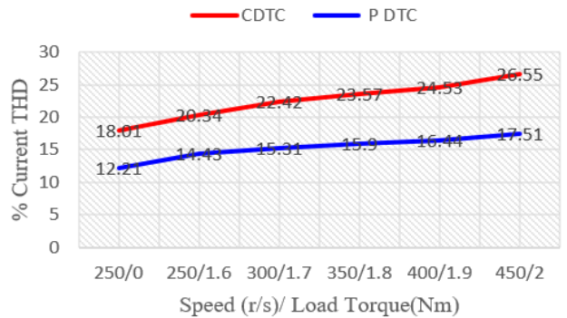
Figure. 12 Comparison of performance indices of % THD of Stator currents
