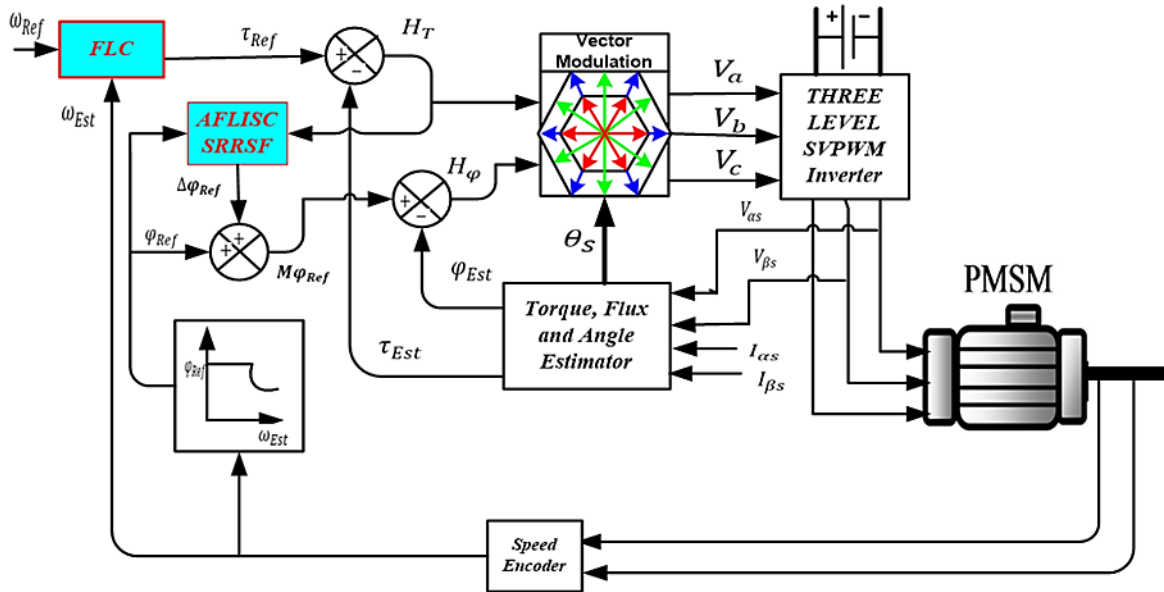
Figure. 6 Simulink orientation block diagram of TH-LI fed DTC of IPMSM
