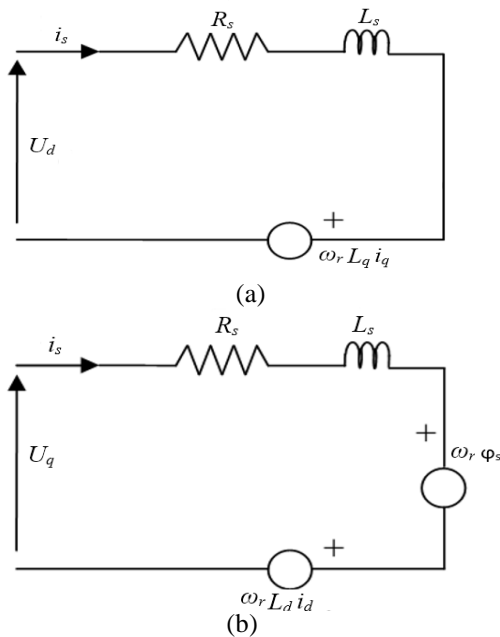
Figure.2 Equivalent circuit of an IPMSM: (a) q axis circuit and (b) d axis circuit
