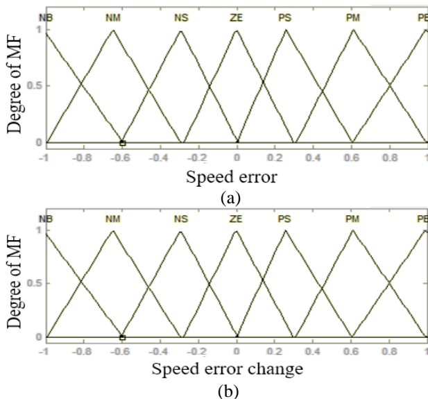
Figure.3 Membership Functions: (a) speed error and (b) change in speed error
