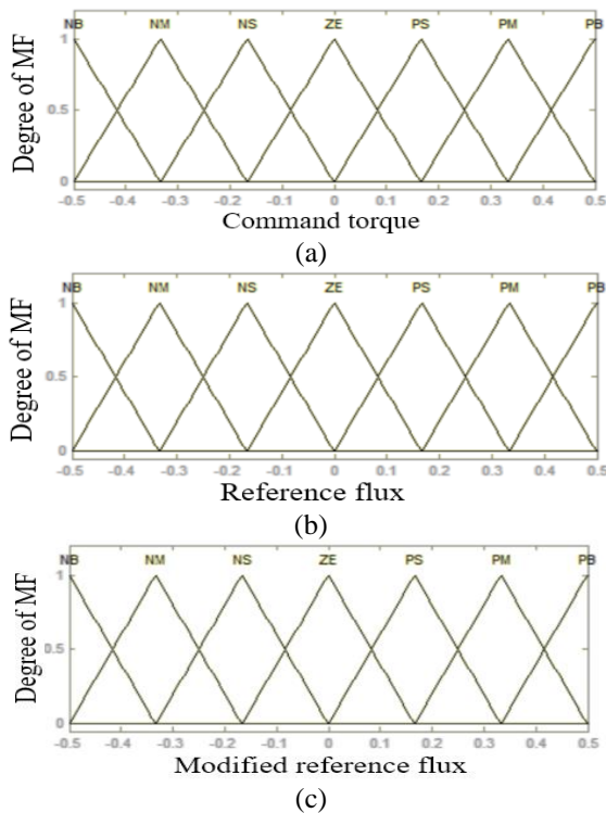
Figure.5 Scaling Factor based MFs: (a) torque error (b) reference stator flux (c) modified stator flux
