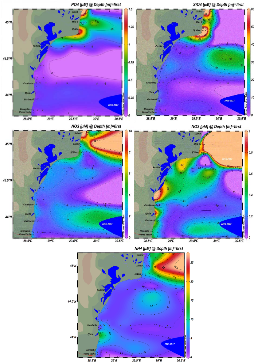
Fig. 2. Nutrients (PO 4 -phosphate, SiO 4 -silicate, NO 3 -nitrate, NO 2 -nitrite and NH 4 -ammonium) surface distribution, Romanian Black Sea, 2015-2017.
