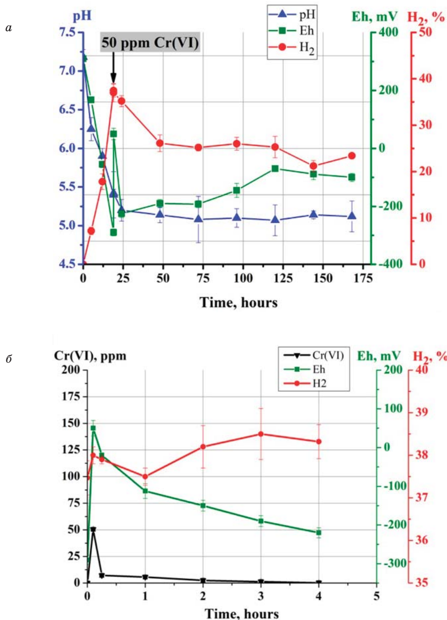
Fig. 6. The dynamics of the reduction of 50 ppm Cr(VI) by the strain Clostridium butyricum GMP1: a — the overall dynamics of the process after addition of Cr(VI); b — the detailed dynamics of Cr(VI) reduction
