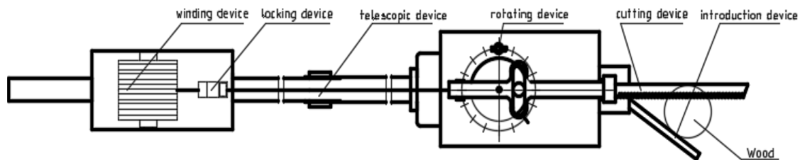
Fig. 1 - Schematic diagram of omni-directional pruning saw
