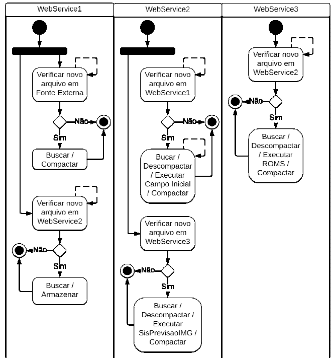
Fig. 5. Activities Diagram
