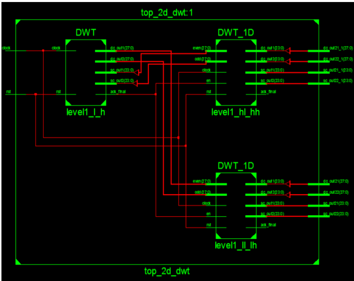
Figure.19 Internal schematic of 2D-DWT
