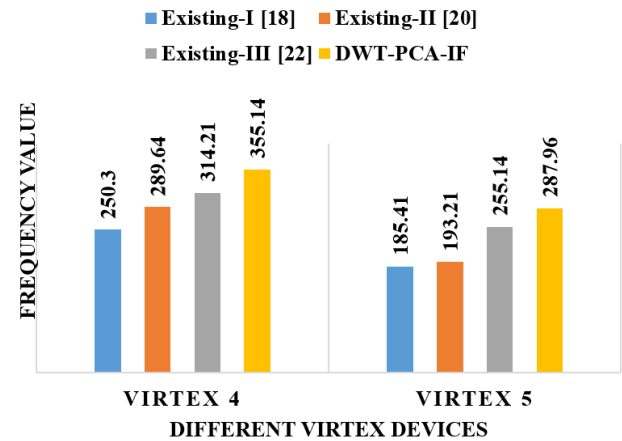
Figure.17 Comparison of Frequency for different methods
