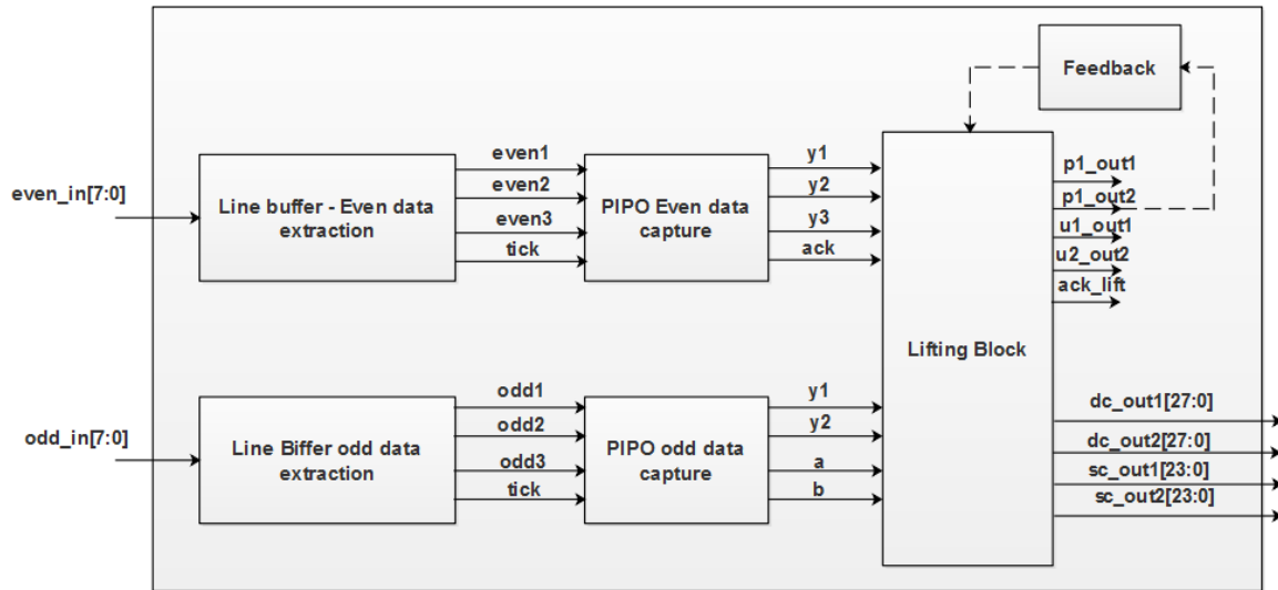
Figure.4 1D- DWT architecture
