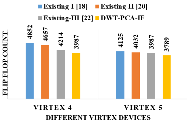
Figure.15 Comparison of flip flop for different methods
