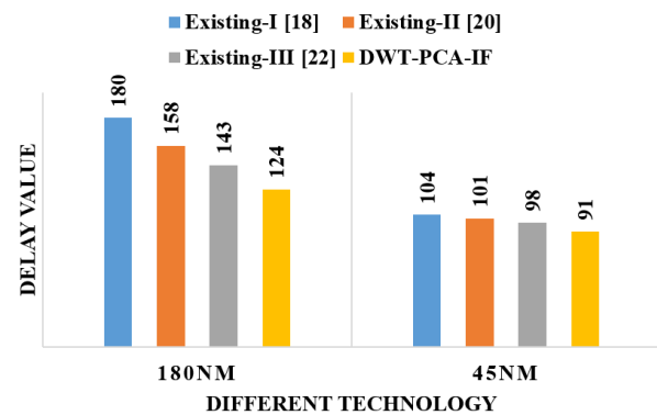
Figure.13 Comparison of delay performance for different methods
