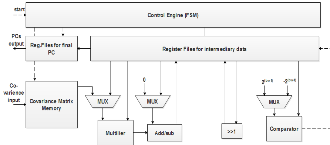
Figure.6 PCA architecture
