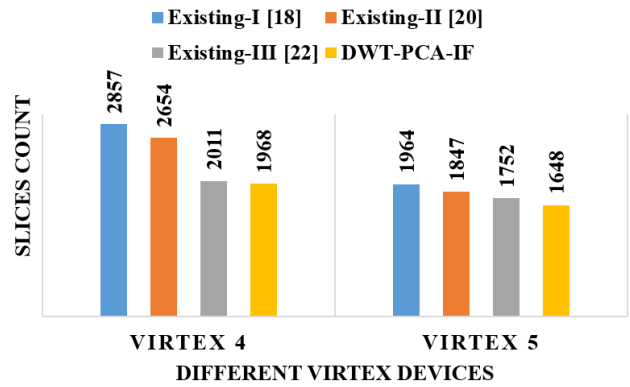
Figure.16 Comparison of slices for different methods
