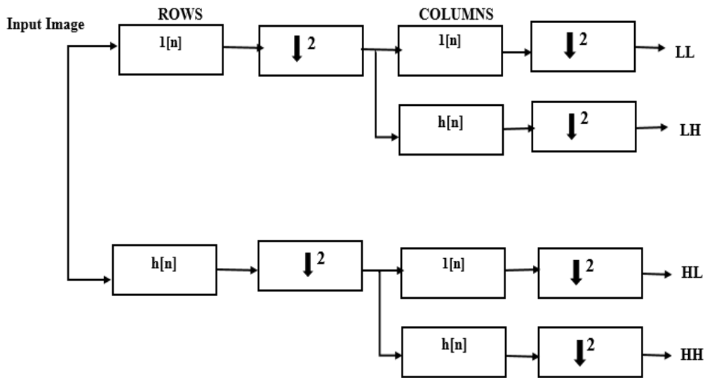
Figure.2 Discrete wavelet transform
