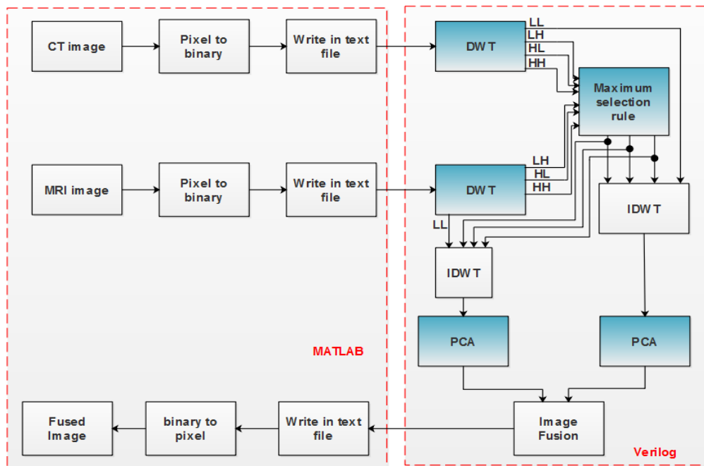
Figure.1 Block diagram of entire process
