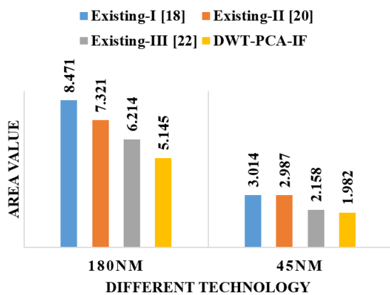
Figure.11 Comparison of area performance for different methods
