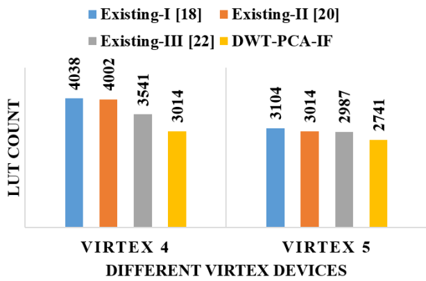
Figure.14 Comparison of LUT for different methods
