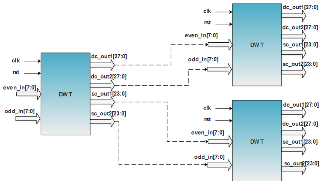
Figure.3 2D- DWT architecture
