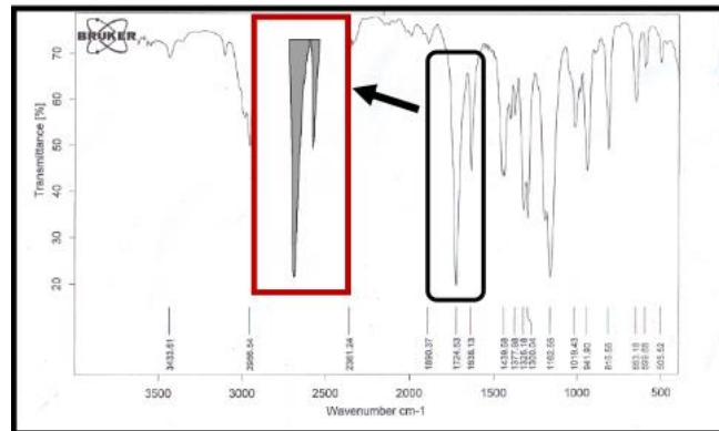
Fig. 5: Infrared spectrometer chart of the monomer (methylmethacrylate)
