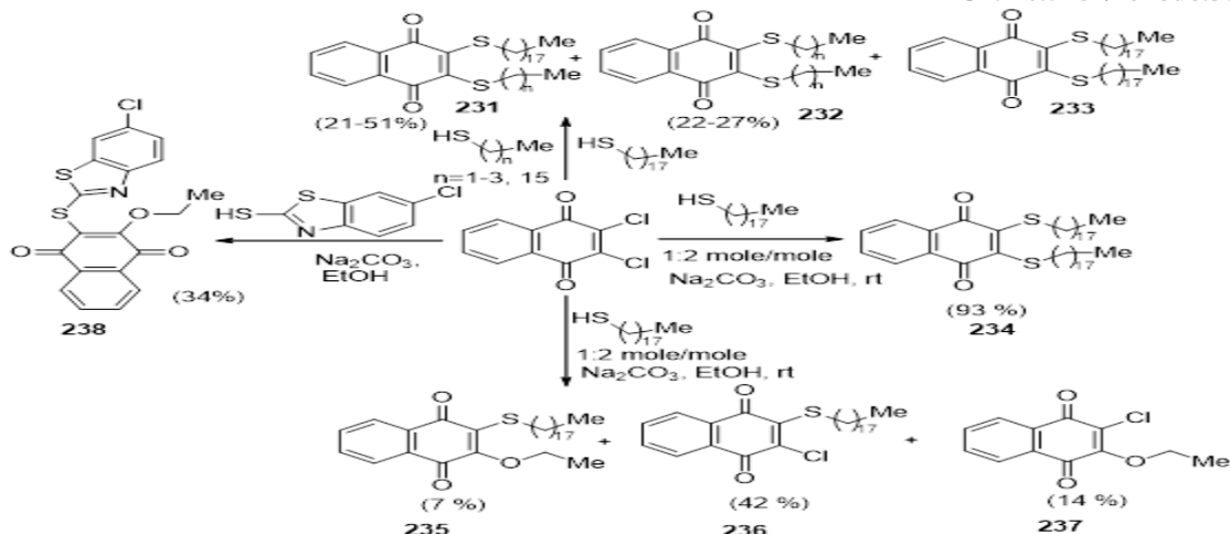
Scheme 49: Synthesis of various sulfur containing naphthoquinones.
