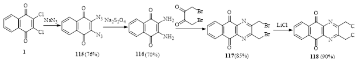
Scheme 25: Synthesis of 2,3-bis(chloromethyl)benzo[g]quinoxaline-5,10-dione (118) from dichloro (1)
