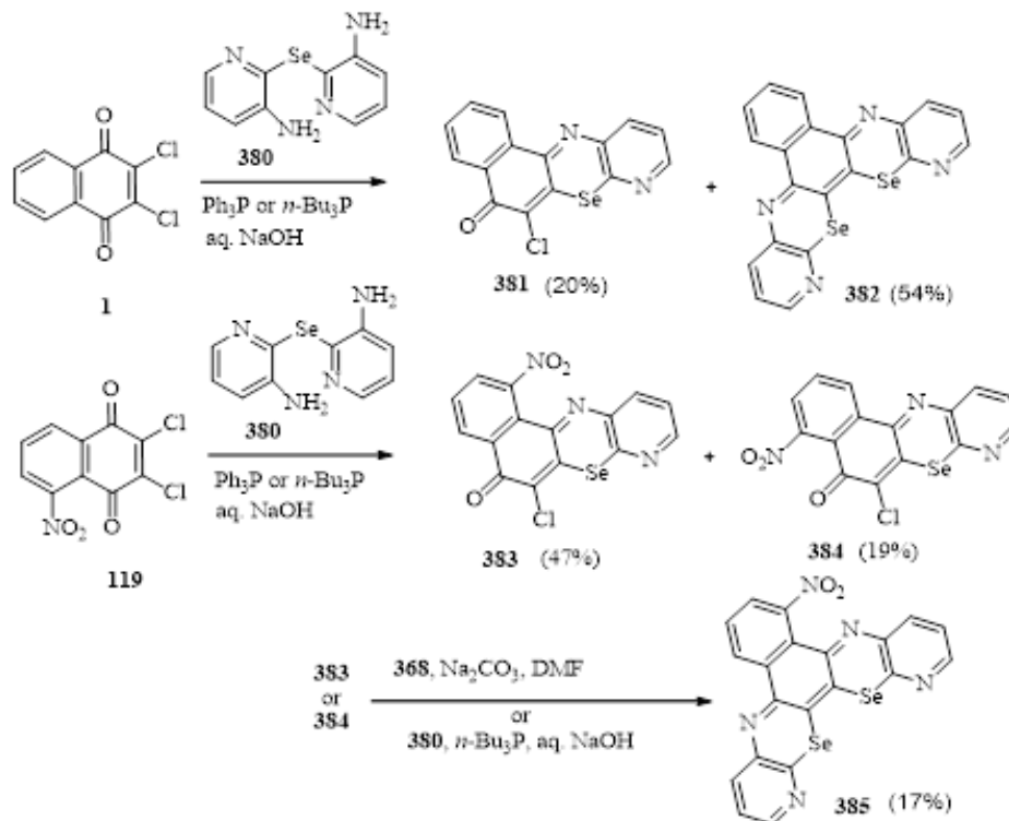
Scheme 77: Synthesis of selenium based heterocycles.
