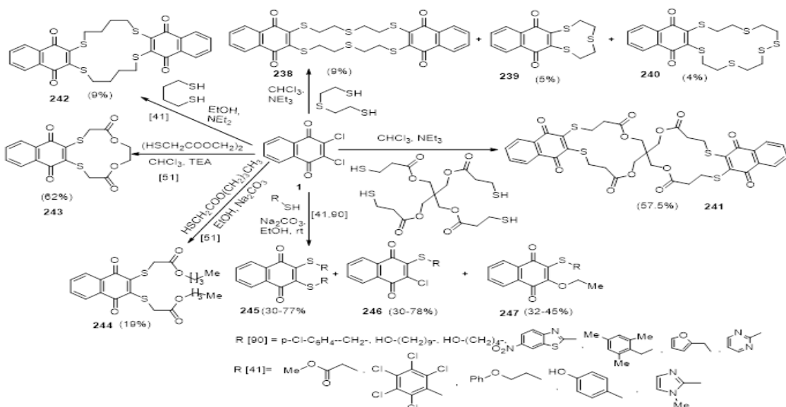
Scheme 50: Synthesis of naphthoquinone fused sulfur containing crown ethers.
