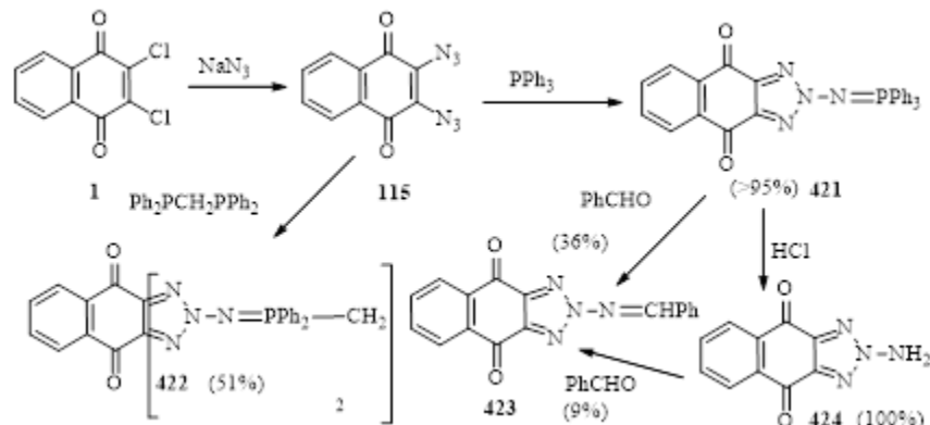
Scheme 91: Synthesis of 2-(benzylideneamino)-2H-naphtho[2,3-d][1,2,3]triazole-4,9-dione
