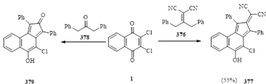
Scheme 76: Synthesis of fulvenes.
