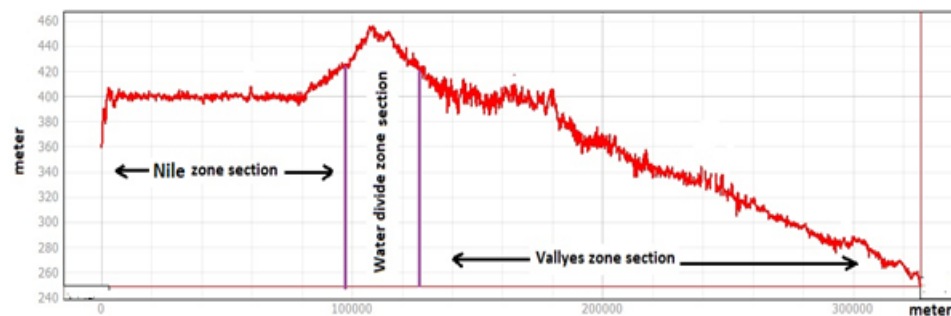
Figure 8, Profile of water course 2.
