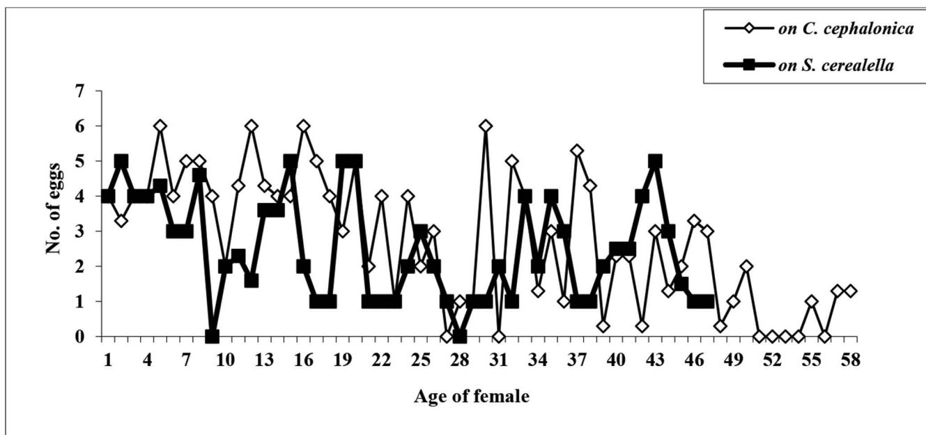
Fig. 1. Day wise fecundity of Blaptostethus pallescens on two alternate laboratory host eggs.
