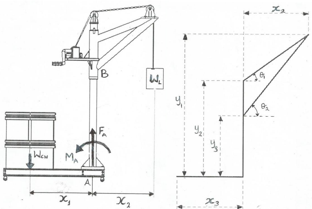
Figure 3: Free Body Diagram of the Crane Figure 4: Dimension of the structural members of the Crane
