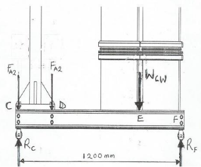
Figure 7: FBD of the Side Frames
