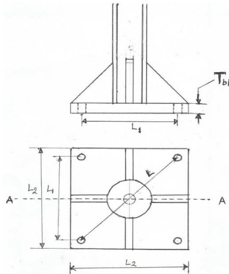
Figure 8: Diagram of the Base Plate for Bolting the Main Support
