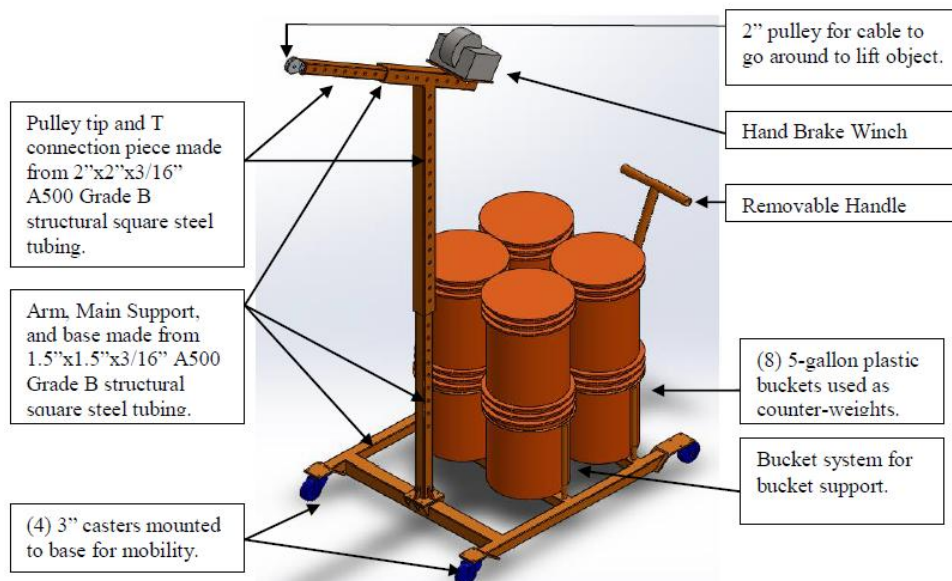
Figure 1: Portable Balcony Crane (Source: [7])
