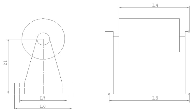
Figure 9: Free Body Diagram of the Hoisting Drum of the Winch
