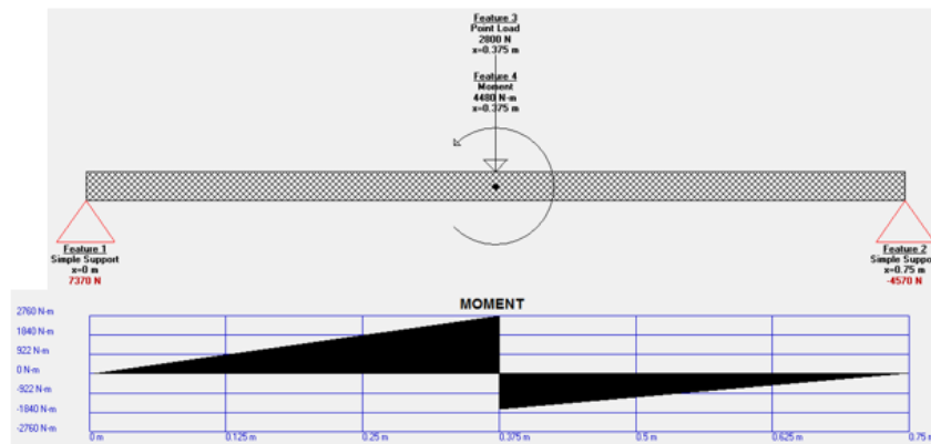
Figure 6: Force Analysis and Bending Moment of the cross piece
