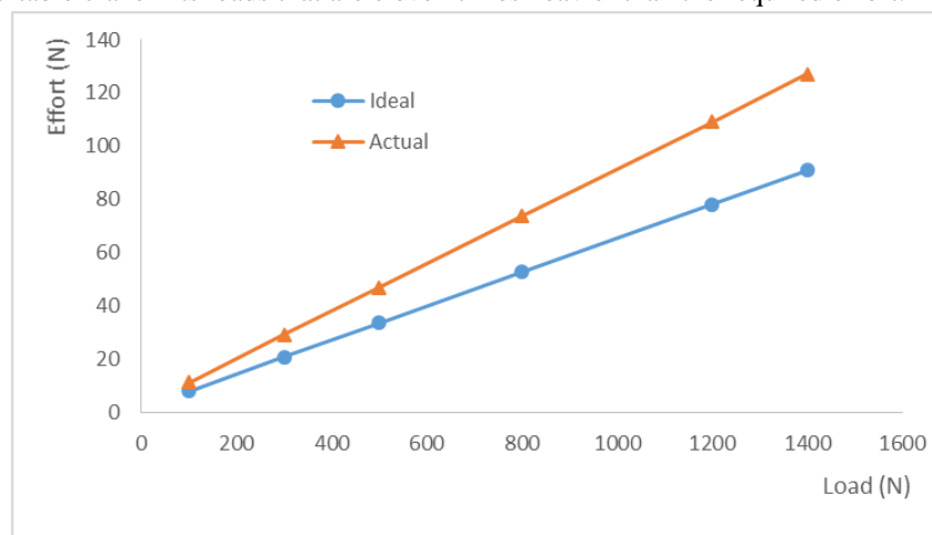
Figure 11: Mechanical Advantage of the Crane
