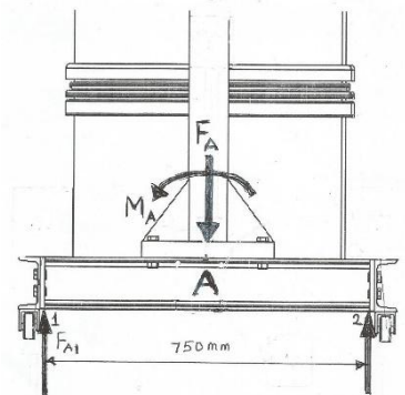
Figure 5: FBD of each front Crosspiece
