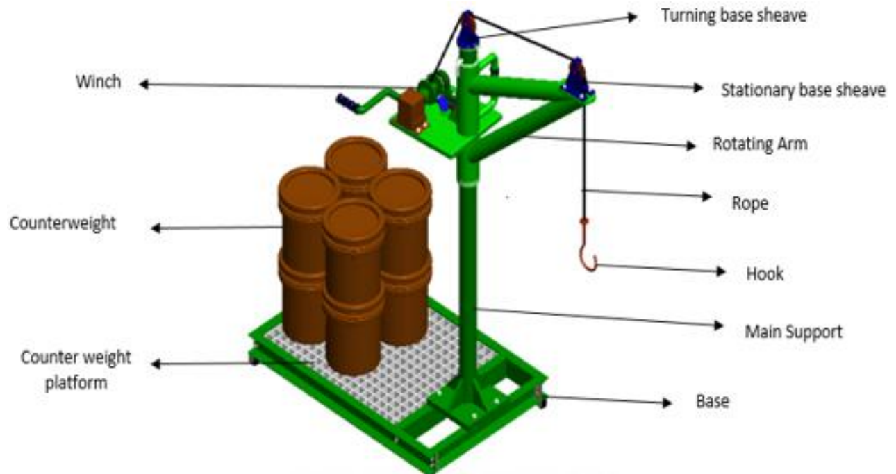
Figure 1: Portable Rotating Arm Balcony Crane
