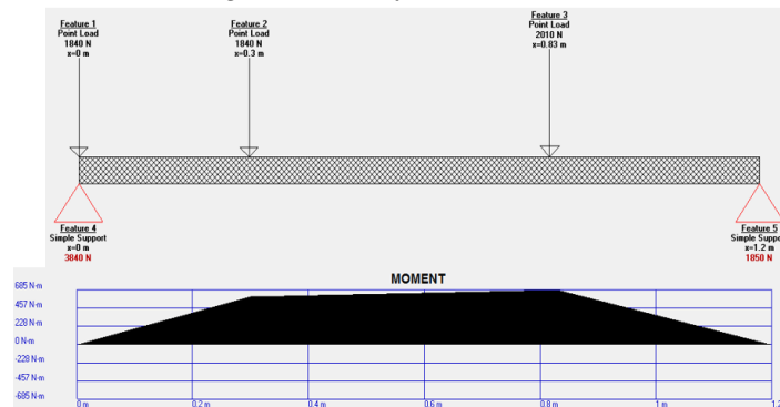
Figure 8: Force Analysis and Bending Moment of the cross piece
