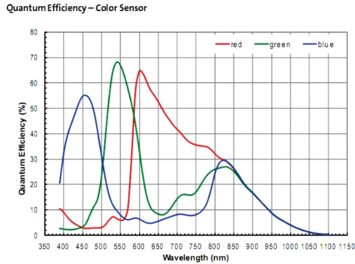
Figure 4. Quantum efficiency of the CMOS sensor (Source: ZWO Optics)
