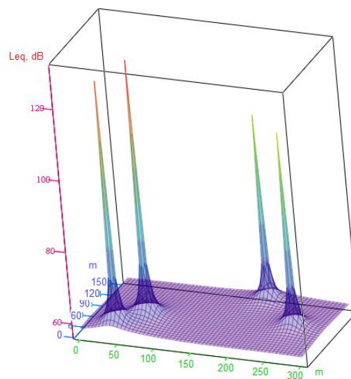
Fig. 19 - Noise field for four tractors (Bulgarian tractors at 1500 rpm and 2000 - left side of the plot and Case tractors, at 1500 and 2000 rpm - right side of the plot).
