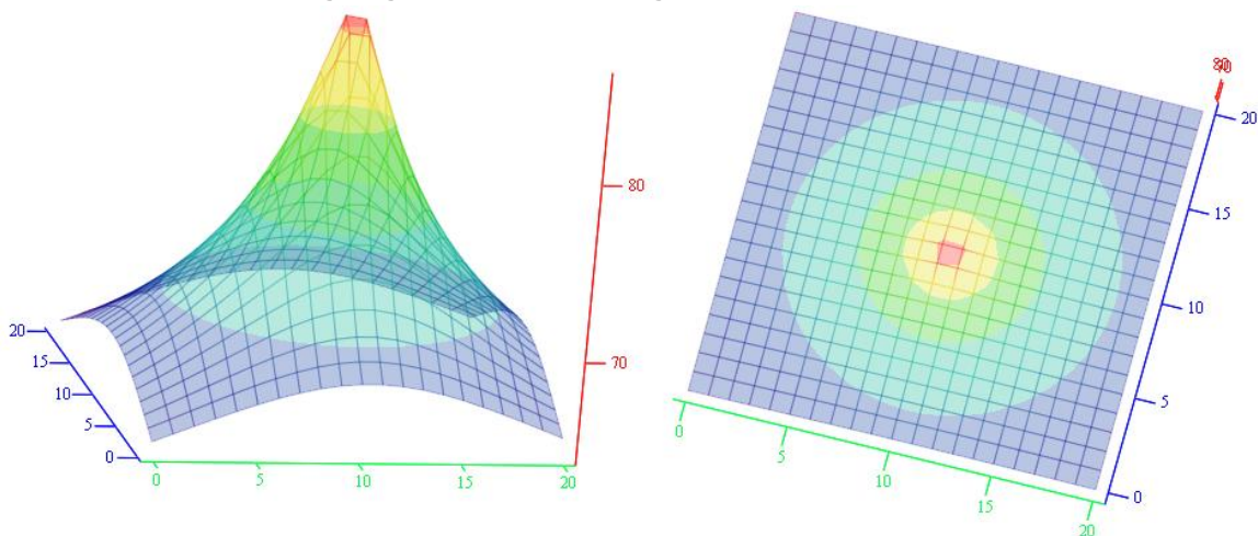
Fig. 12 - Interpolated noise level distribution for Case tractor at 1500 RPM (two projections) at the measuring height of 1.2 m from the ground of the Sound Level Meter
