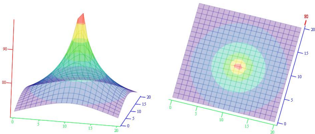
Fig. 11 - Interpolated noise level distribution for Bulgarian tractor at 2000 RPM (two projections) at the measuring height of 1.2 m from the ground of the Sound Level Meter
