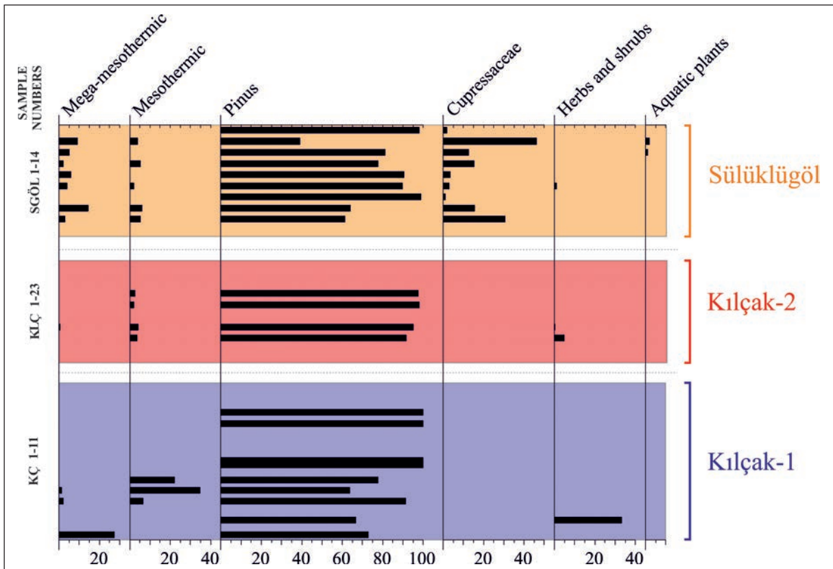
Figure 10- Synthetic pollen diagram of Kılçak-1, Kılçak-2 and Sülüklügöl stratigraphic sections.1. Mega-mesothermic (=subtropical) elements (Taxodioidae, Engelhardtioidae, Carya ); 2. Mesothermic (=warm-temperate) elements (deciduous Quercus , Pterocarya , Carpinus , Juglans , Ulmus , Alnus , Salix , Oleaceae, Castanea – Castanopsis type); 3. Pinus and poorly preserved Pinaceae; 4. Cupressaceae; 5. Herbs and shrubs (Poaceae, Asteraceae/Cichorioideae, Brassicaceae, Chenopodiaceae/Amaranthaceae, Dipsacaceae); 6. Aquatic plants ( Sparganium ).
