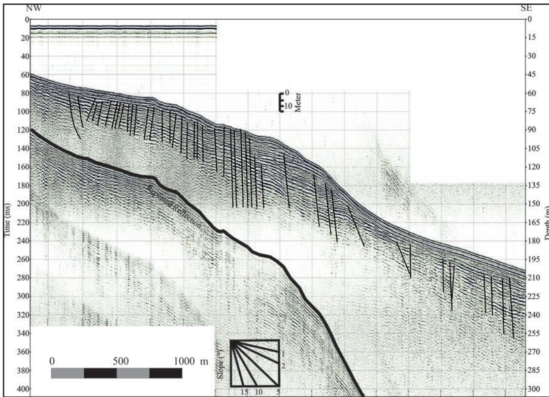
Figure 10- Seismic reflection profile no. 10 from east of Datça Bay. For section location see figure 6, interpretation in text.
