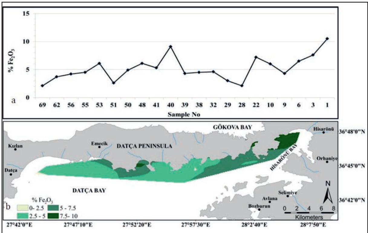
Figure 25- a) \text{Fe}_2\text{O}_3 amounts and b) \text{Fe}_2\text{O}_3 spatial distribution in surface sediments in Datça-Hisarönü Bays.
