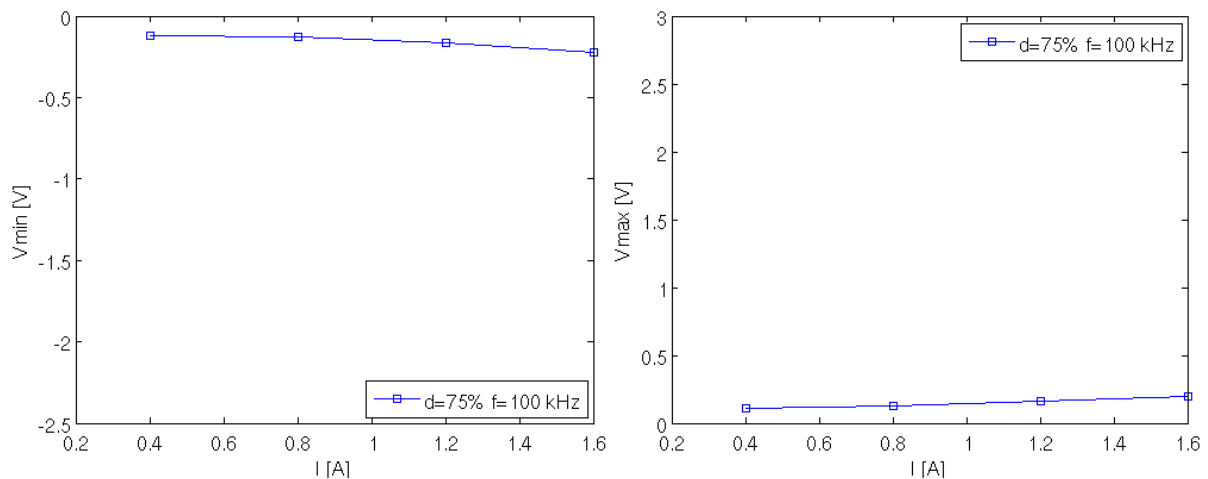
Fig. 7. Output voltage peaks for different currents with the usage of solenoid, for a) minimum voltage peaks, b) maximum voltage peaks Source: Author's
