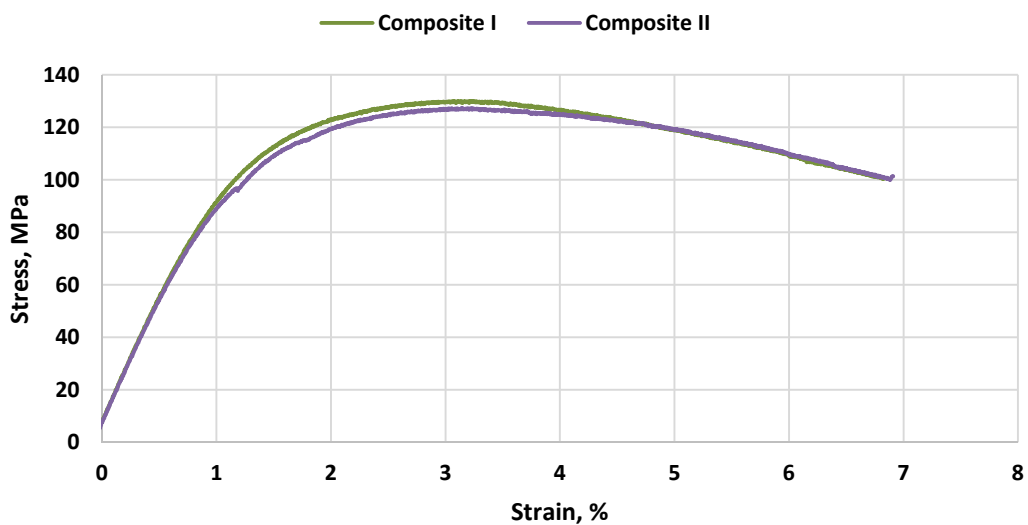
Fig. 6. Results of tensile bending investigations of polyamide of composites Source: Author's
