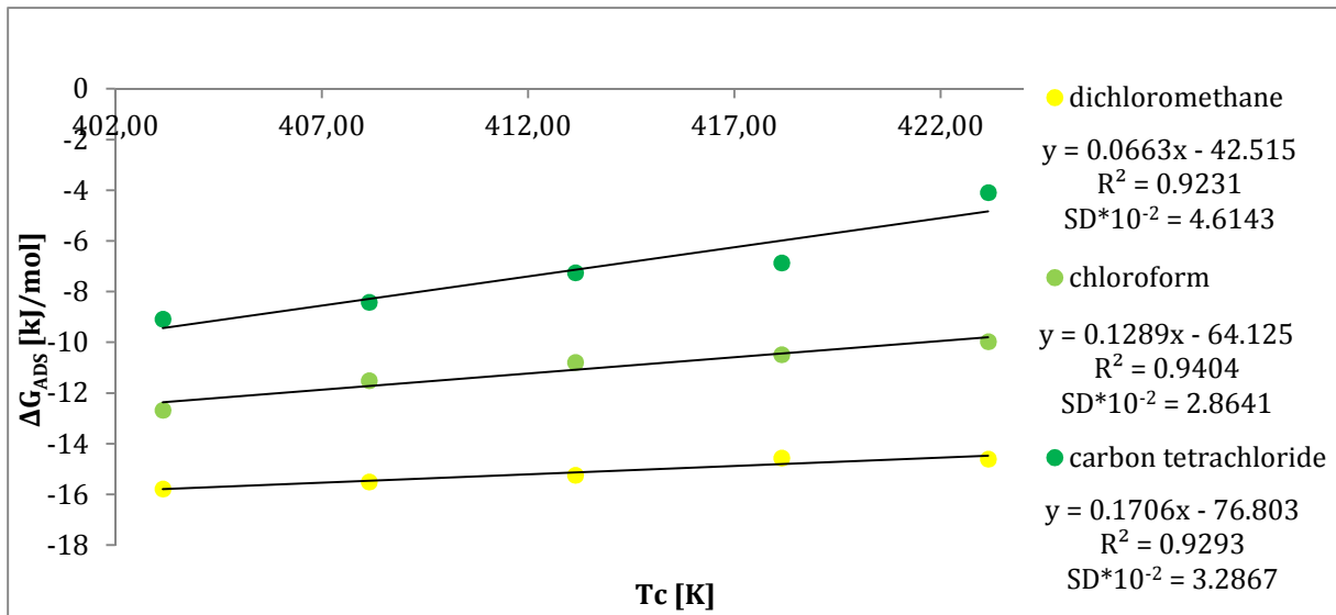
Fig. 9. The -\Delta G_{\text{ADS}}=f(T_c) dependency for GO (dichloromethane, chloroform, carbon tetrachloride; the ExtraVal4T function) Source: Author's
