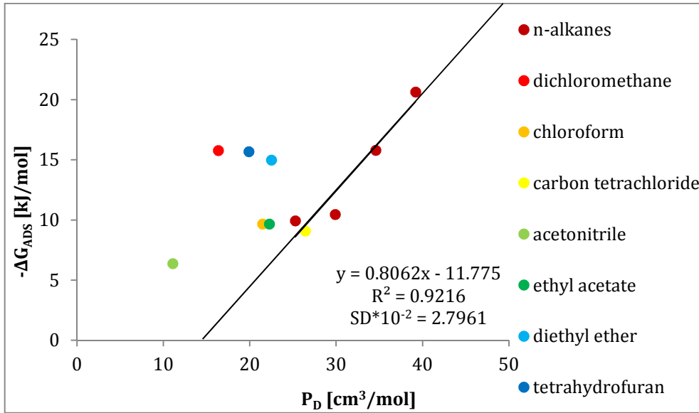
Fig. 12. The \Delta G_A = f(P_D) dependency for GO (the ExtraVal4T function) Source: Author's
