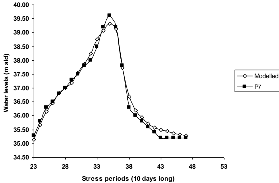
Figure 8: Observed and modelled groundwater heads for node (27, 2) mald = meters above local datum
