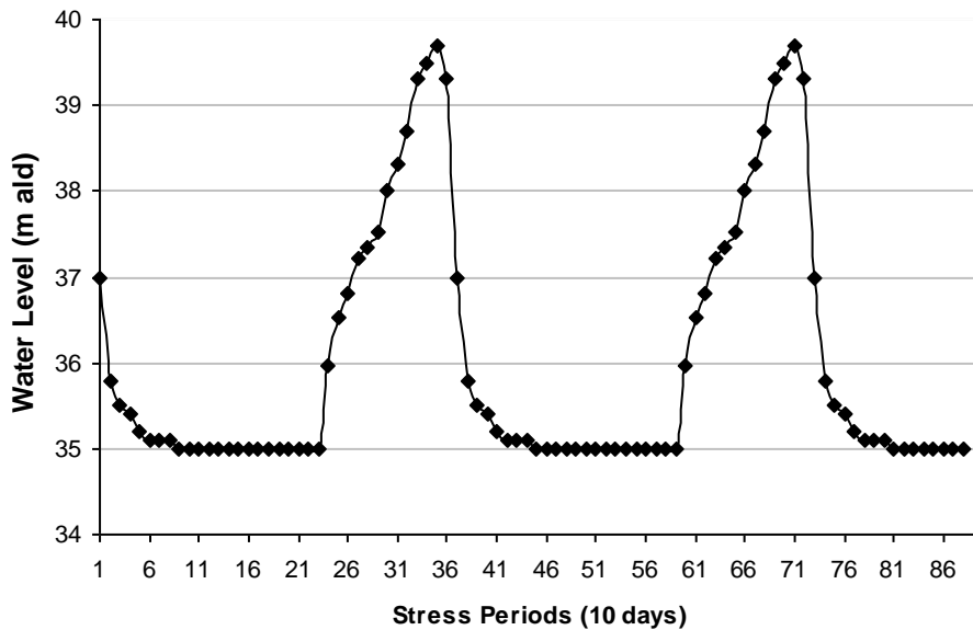
Figure 5: River stage variations with time
