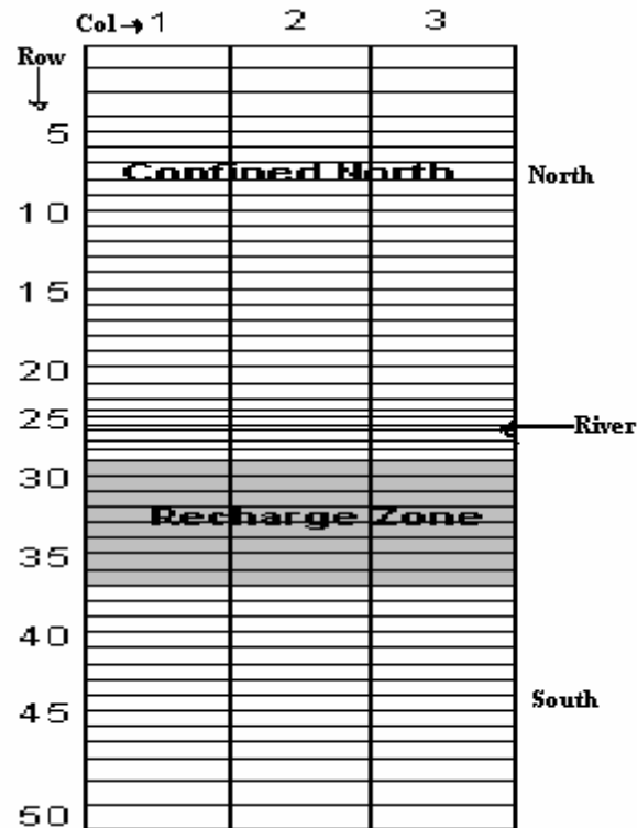
Figure 7: Finite difference grid of area of interest showing recharge area
