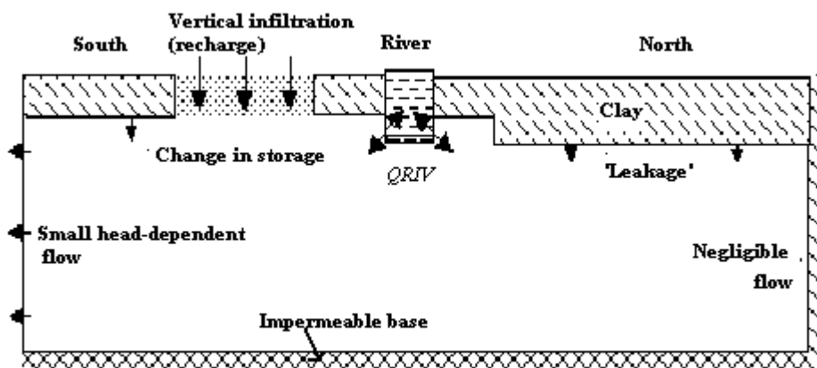
Figure 2: Conceptual model of the Yobe river system
