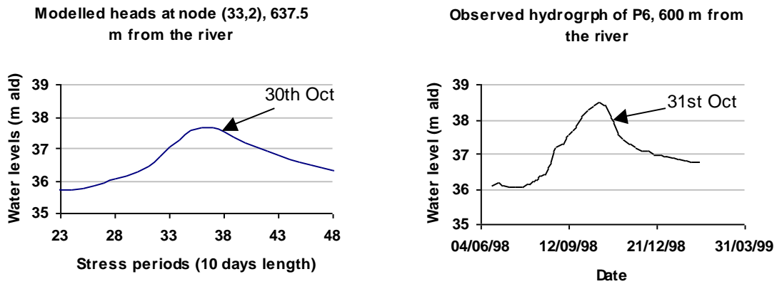
Figure 9: Groundwater heads at 600 m south of the river; (a) modelled, (b) observed mald = meters above local datum
