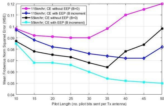
Figure. 6 Impact of CE with/without EEP for \mu = 55\text{km/hr} and 115\text{km/hr} channels
