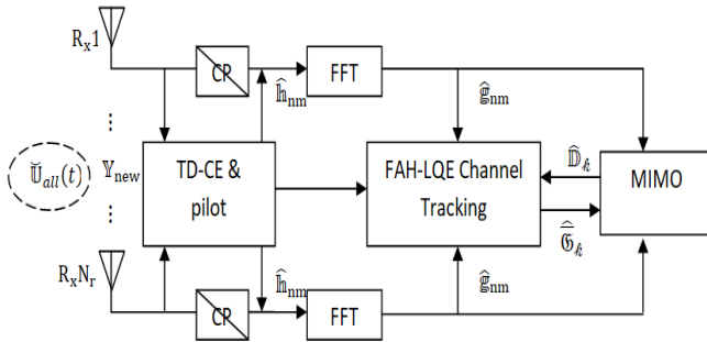
Figure. 2 Receiver block diagram for proposed EEP-CE and FAH-LQE-CT
