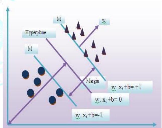
Figure 5. Hypeplane with margins for SVM
