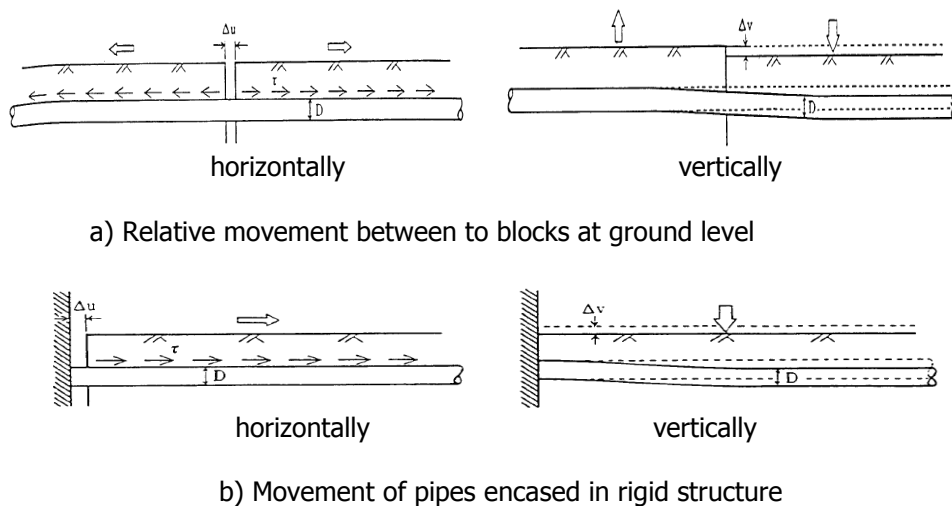
Figure 3. Pipes deformation caused by ground movement [33] ( \Delta u - horizontal deformability index, \Delta v - vertical deformability index, \tau –ground restraint)
