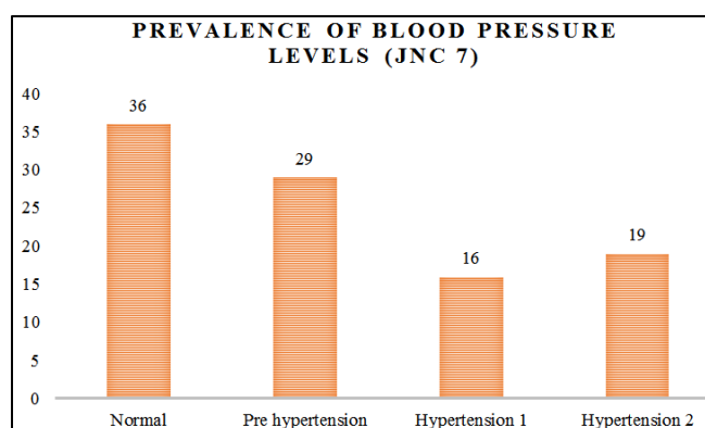
Fig. 1: Prevalence of blood pressure levels (JNC 7)
