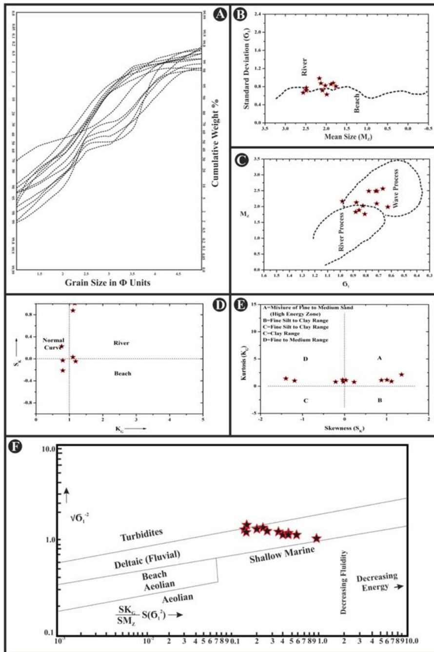
Figure 5 | A. Cumulative grain size curves, B. Binary plot of Graphic Mean ( M_z ) vs Standard Deviation ( \sigma_1 ) 15 representing the depositional conditions, C. Binary plot of Mean Size ( M_z ) vs Standard Deviation ( \sigma_1 ) 16 suggesting the sediments were deposited by wave processes, D. Skewness ( S_{ki} ) vs Kurtosis ( K_G ) plot 17 representing the depositional condition of sediments, E. Binary plot of Skewness ( S_{ki} ) vs Kurtosis ( K_G ) 18 to depict the energy conditions, F. Log-Log plot 19 showing the depositional environment.
