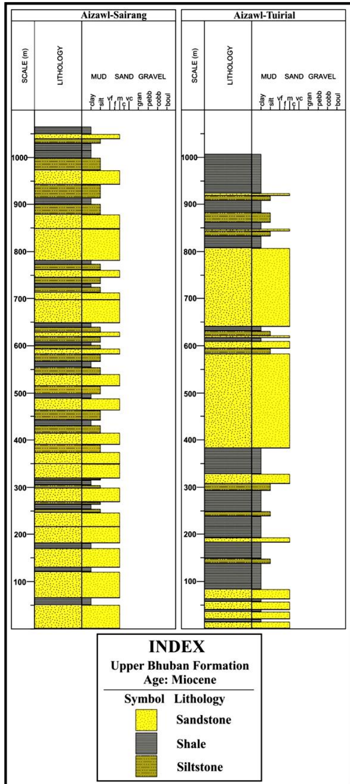
Figure 2 | Lithocolumn of the studied sections.
