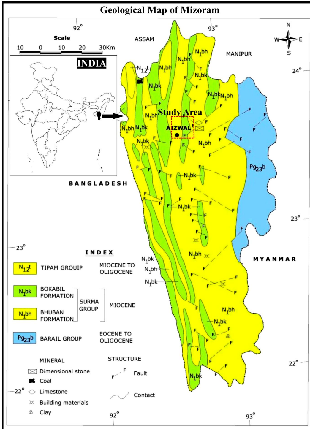
Figure 1 | Geological map of Mizoram showing the study area. 21
