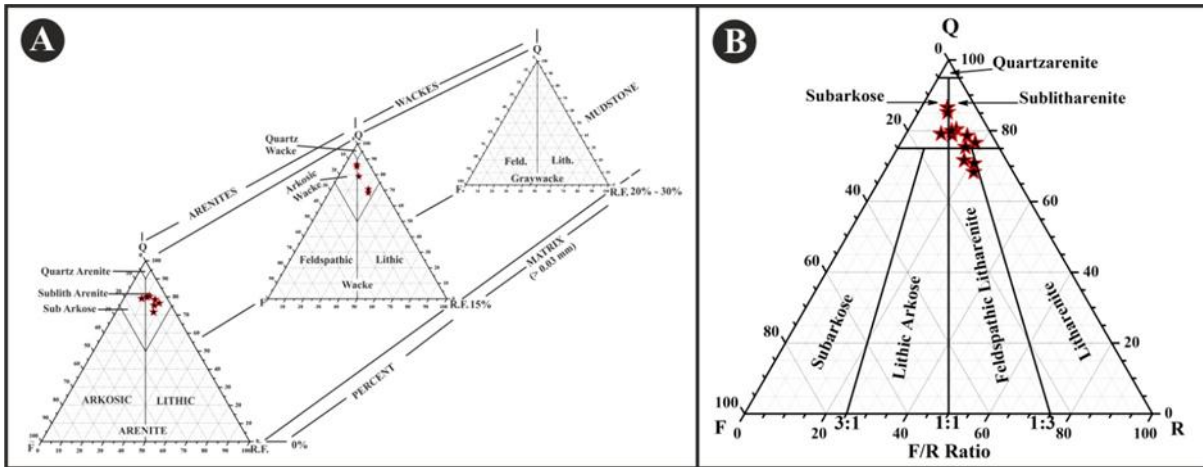
Figure 8 | Petrographic classification of sandstones. A. QFL. 30 B. QFR. 31
