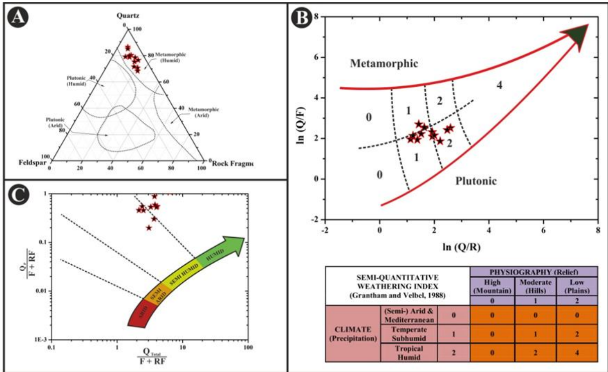
Figure 10 | Paleoclimatic conditions of Upper Bhuban Formation – A. Ternary QFR plot 45 representing humid climatic condition. B. Semi Quantitative Weathering Index 11 and binary plot of \ln(Q/R) vs \ln(Q/F) 46 representing moderate nature of weathering. C. Bivariate plot 12 of modal data representing humid to semi humid climatic conditions.
