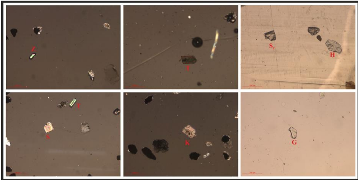
Figure 6 | Heavy minerals observed under microscope (where, Z: zircon, T: tourmaline, S T : staurolite, H: hypersthene, R: rutile, S: sillimanite, K: kyanite & G: garnet).
