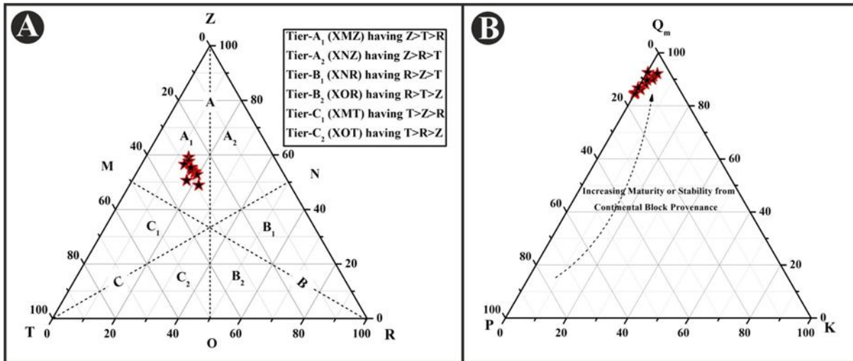
Figure 7 | A. ZTR index 29 of Upper Bhuban sandstones. B. Q m PK ternary plot 44 representing continental derivation of sediments with increasing maturity index.
