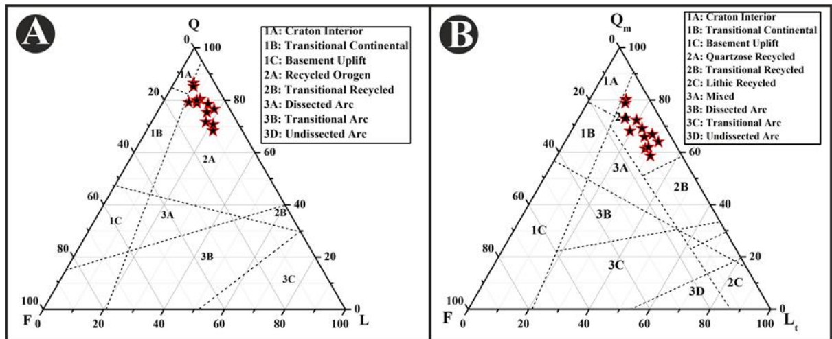
Figure 11 | Petrographic tectonic setting discriminant plot – A. QFL ternary plot. 9 B. Q_mFL_t ternary plot 10 representing recycled orogen and quartzose recycled orogen.
