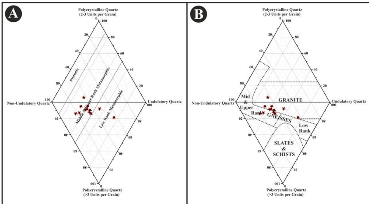
Figure 9 | Monocrystalline and polycrystalline quartz are plotted in - A. Diamond Diagram 7 representing the derivation of sediments from upper to middle rank metamorphic rocks; B. Diamond Plot 8 representing derivation of sediments from granite and gneisses.
