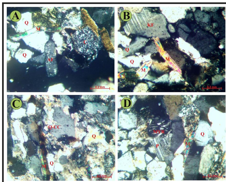
Figure 4 | Photomicrographs of Upper Bhuban sandstone (where, Q: Quartz, P: Plagioclase, KF: K-Feldspar, M: Mica, AF: Altered Feldspar, C: Chert, RF: Rock Fragment, MYR: myrmekite & Q-CC: quartz overgrowth with carbonate cement).
