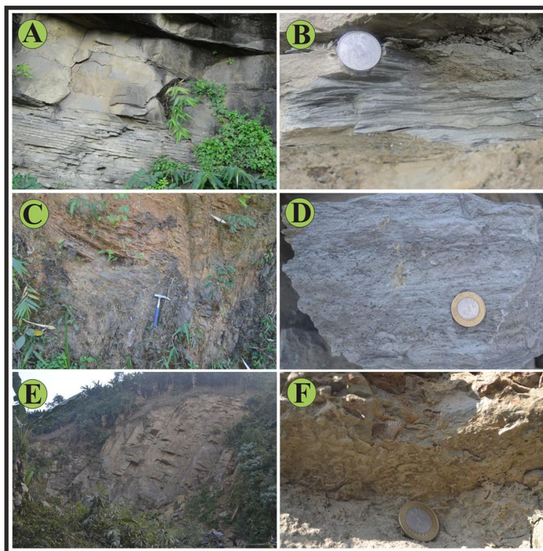
Figure 3 | Field photographs of the study area. A: Massive sandstone bed with alternate bands of sandstone and siltstone along Aizawl-Sairang road section, B: Siltstone intercalations between sandstone beds, C: Chevron folding observed along Aizawl-Sairang road section, D: Bioturbation developed within sandstone, E: jointed steep sandstone beds along Aizawl-Tuirial road section and F: bivalves associated with weathered sandstone beds along Aizawl-Sairang road section.
