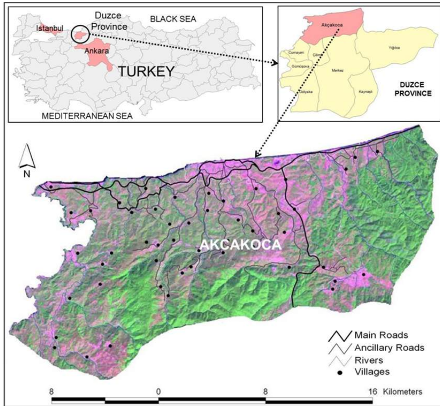
Figure 1. Geographical location of Akcakoca district.
