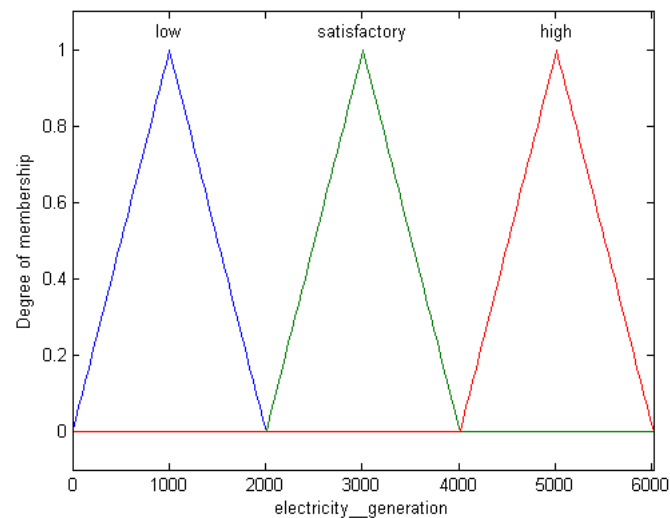
Figure 5: The three membership functions (low, satisfactory, high) for the output variable “annual electricity’s generation”
