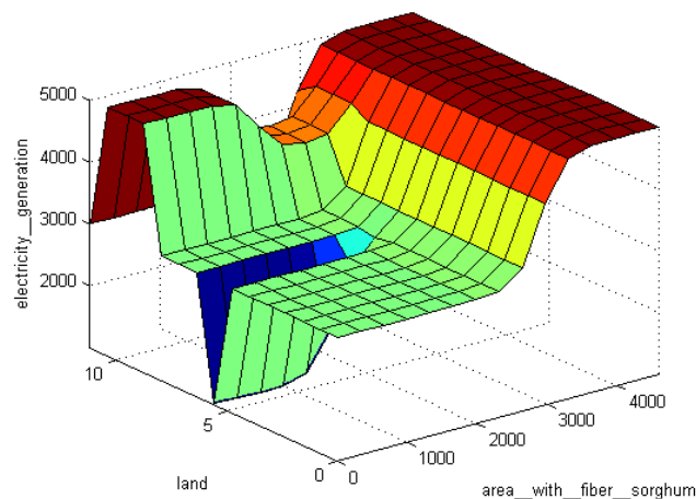
Figure 8: The surface viewer: annual electricity’s generation as it is affected by the cultivating area with fibre sorghum and land’s yield
