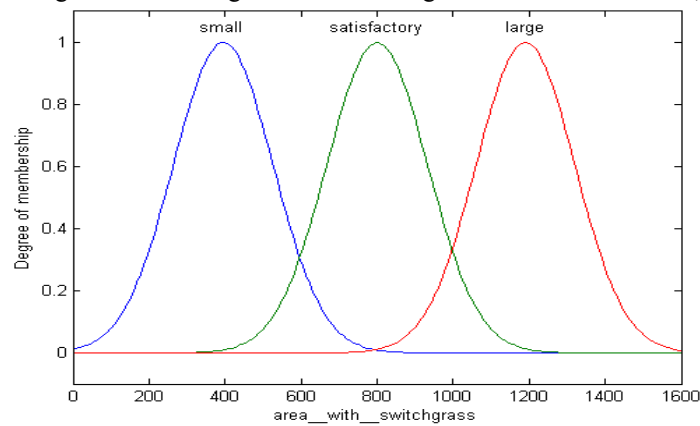
Figure 4: The three membership functions (small, satisfactory, large) for the input 1 variable “cultivating area with switchgrass”
