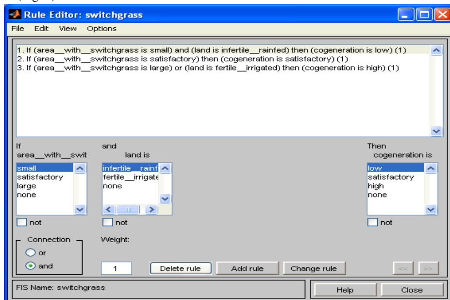
Figure 7: The rule editor: the three rules are appeared in the up part of this window
