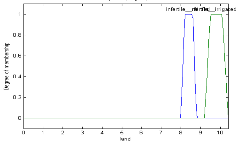
Figure 5: The two membership functions (infertile rainfed, fertile irrigated) for the input 2 variable “land’s yield”
