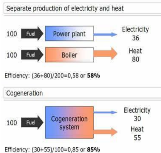
Figure 1: Efficiency of Cogeneration and Separate production of electricity and heat
