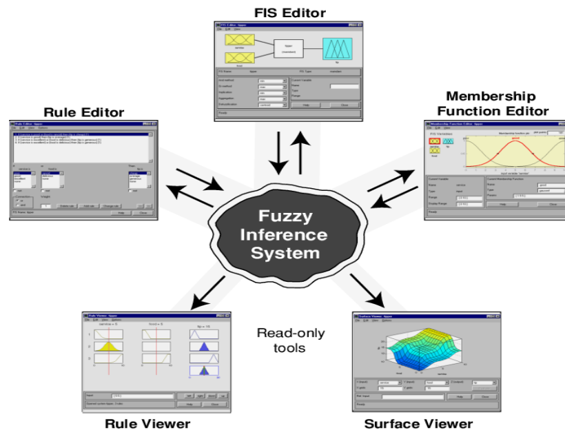
Figure 2: A Mamdani-type fuzzy inference system using the Fuzzy Logic Toolbox Graphical User Interface (GUI) Tools. The Membership Function Editor (top right), FIS Editor (center), Rule Editor (top left), Rule Viewer (bottom left) and Surface Viewer (bottom right).
