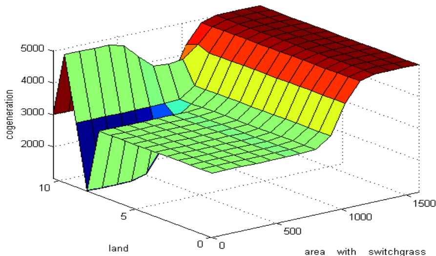
Figure 9: The surface viewer: annual cogeneration as it is affected by the cultivating area with switchgrass and land’s yield
