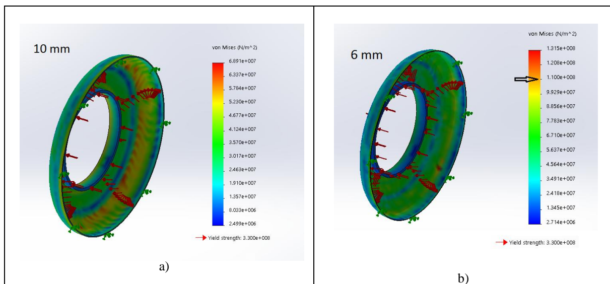
Figure 8: Stress analysis results of torispherical head a) s=10 mm (calculated) b) s=6 mm (suggested)
