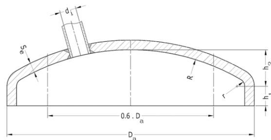
Figure 3: Geometrical dimensions of torispherical head
