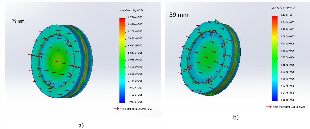
Figure 11: Stress analysis results of porthole flange a) s=80\text{ mm} (calculated) b) s=59\text{ mm} (suggested)
