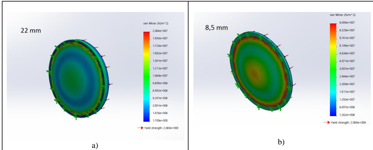
Figure 10: Stress analysis results of medical lock outside wall a) s=22\text{ mm} (calculated) b) s=8.5\text{ mm} (suggested)
