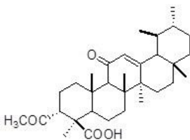
Fig.4 (3R, 4R, 6aR, 6bS, 8aR, 11R, 12S, 14bS)-3-acetyl-4, 6a, 6b, 8a, 11, 12, 14b-heptamethyl-14-oxo-1,2,3,4,4a,5,6,6a,6b,7,8,8a,9,10,11,12,12a,14,14a, 14b-icosahydricene-4-carboxylic acid
