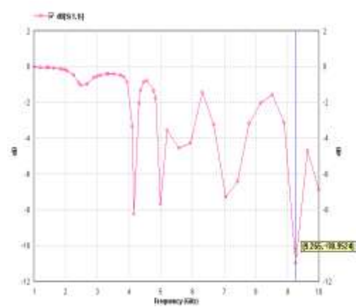
Fig11 Return loss vs frequency of iteration III for proposed antenna
