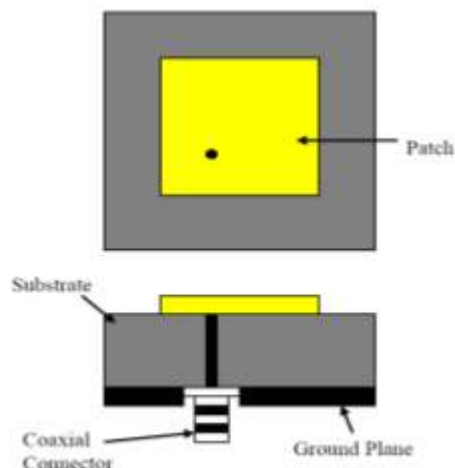
Fig 1 Schematic diagram of Probe-fed Microstrip Patch Antenna
