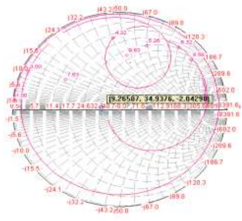
Fig9 Input impedance loci using smith chart of iteration II
