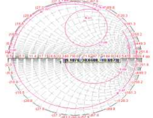
Fig 13 Input impedance loci using smith chart for iteration III
