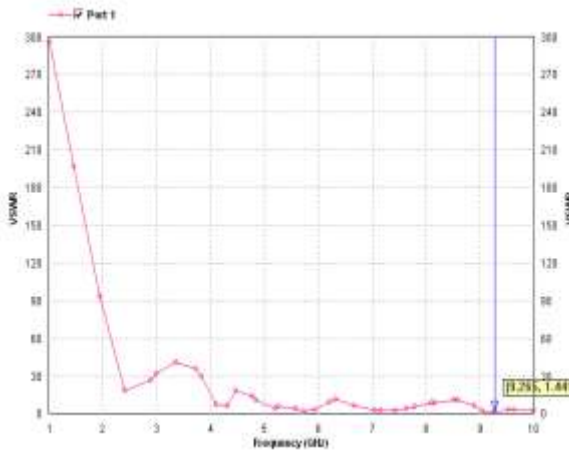
Fig 8 VSWR vs Frequency curve of iteration II for proposed antenna
