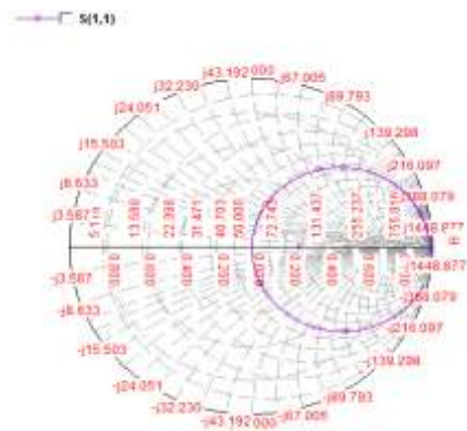
Fig5 Input impedance loci using smith chart of iteration I
