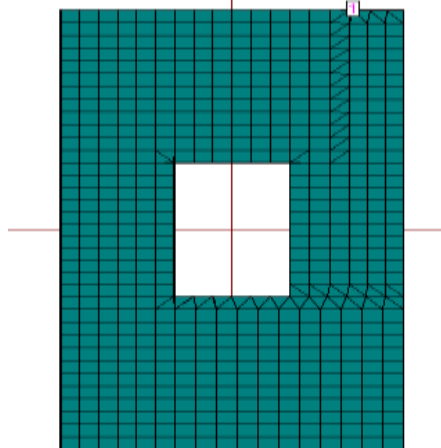
Fig 2 Geometry of iteration 1 with t=16 , Permittivity=22 and grid size=025
