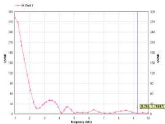
Fig12 VSWR vs Frequency curve of iteration III for proposed antenna
