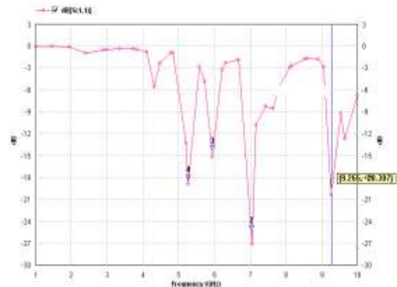
Fig 3 Return loss vs Frequency curve of iteration I for proposed antenna
