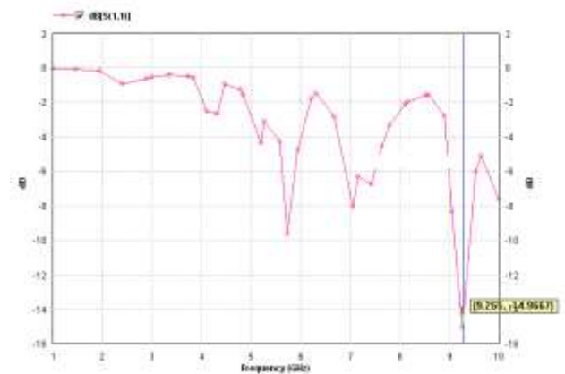
Fig7 Return loss vs Frequency curve of iteration II for proposed antenna
