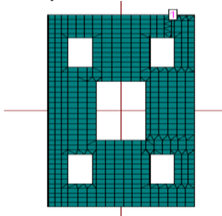
Fig 6 Geometry of iteration II for proposed antenna
