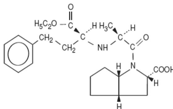
Fig. 2: Molecular structure of Ramipril
