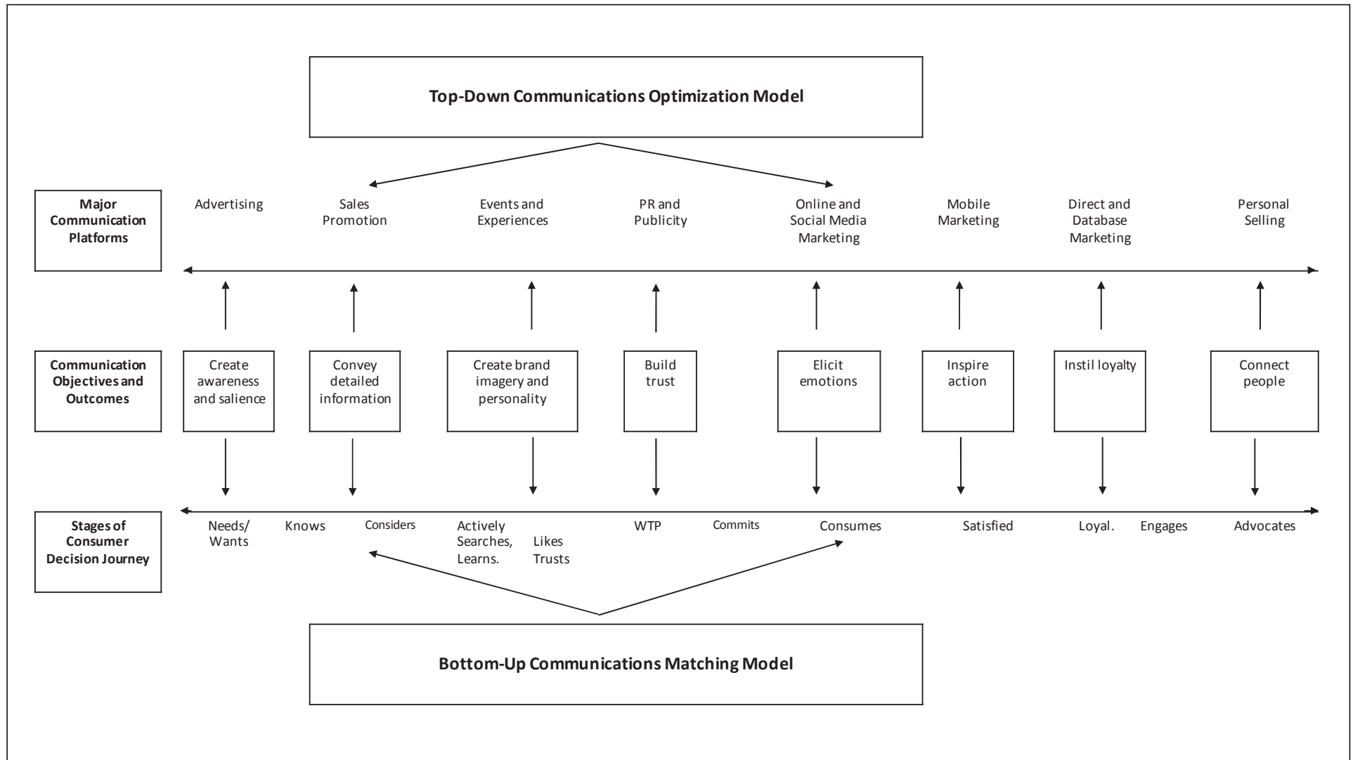
Figure 2 | IMC Framework
