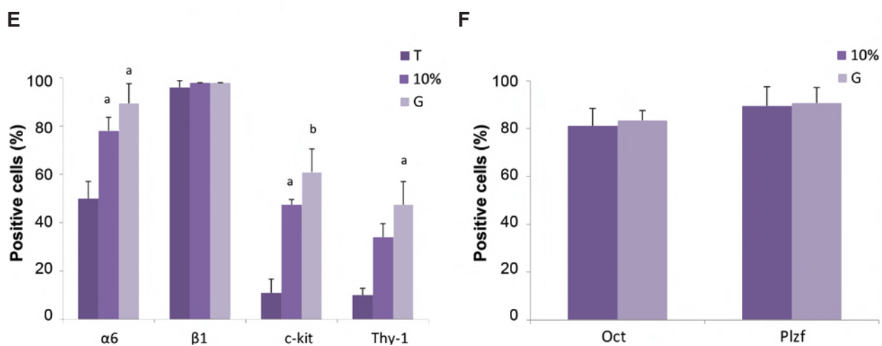
Fig.2: Characterization of spermatogonial stem-like colonies. Immunocytochemistry results showed that spermatogonial stem-like colonies expressed germ cell markers: A. \alpha 6 -Integrin, B. Oct4, C. Plzf, D. c-Kit, E. Flow cytometry analyses for expression of surface markers: \alpha 6 -Integrin, \beta 1 -Integrin, c-Kit, and Thy-1 in the testis (T), 10%, and G groups, and F. Flow cytometry analyses for expressions of Oct4 and Plzf transcription factor in the 10% and G groups. a; P < 0.05 versus the T group and b; At least P < 0.005 versus the T group.
